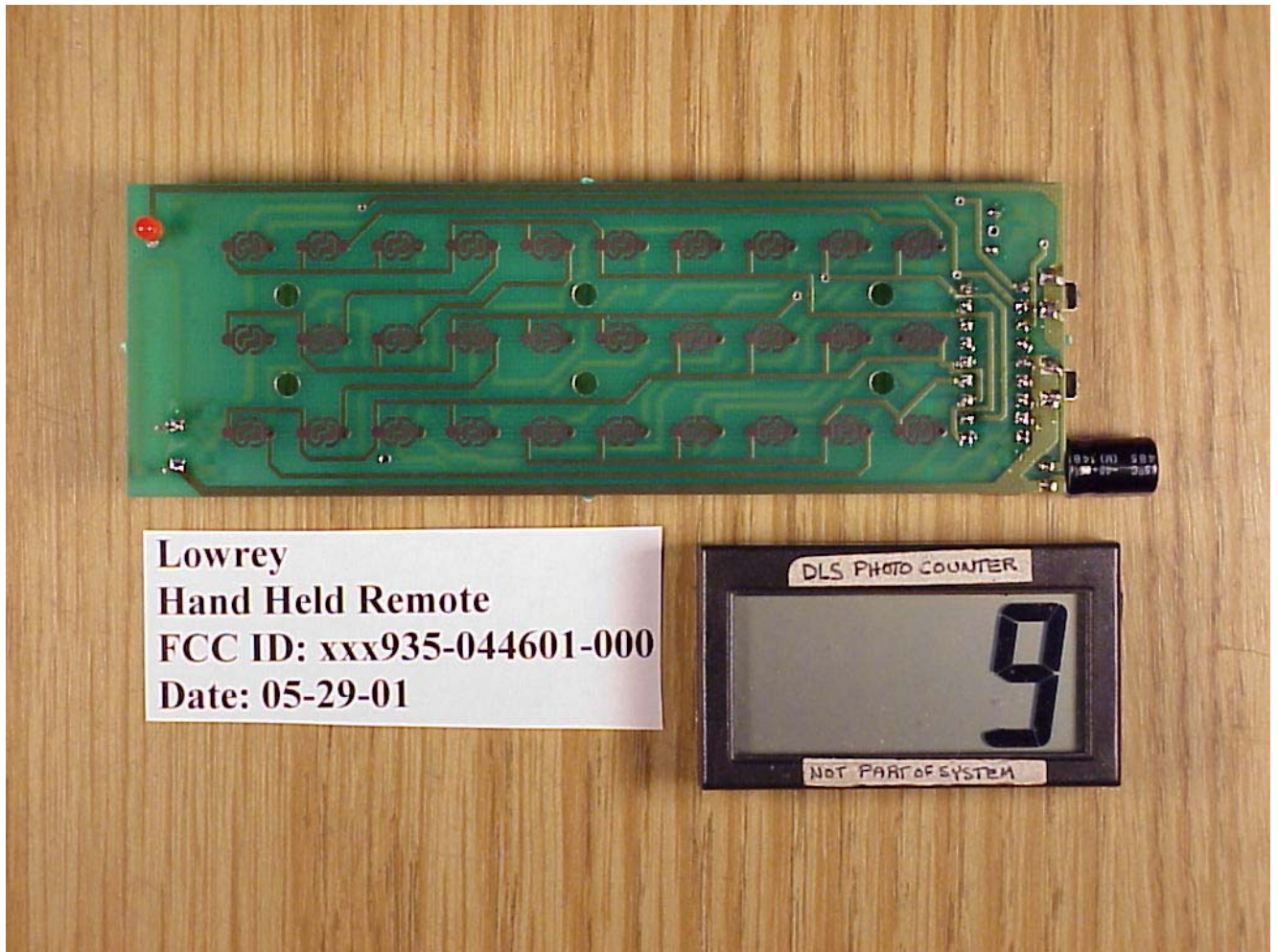
PC Board - Solder Side
