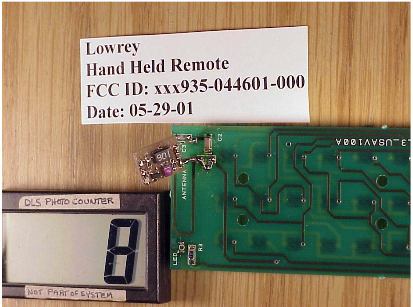
PC Board - Component Side Close up of RF Module
