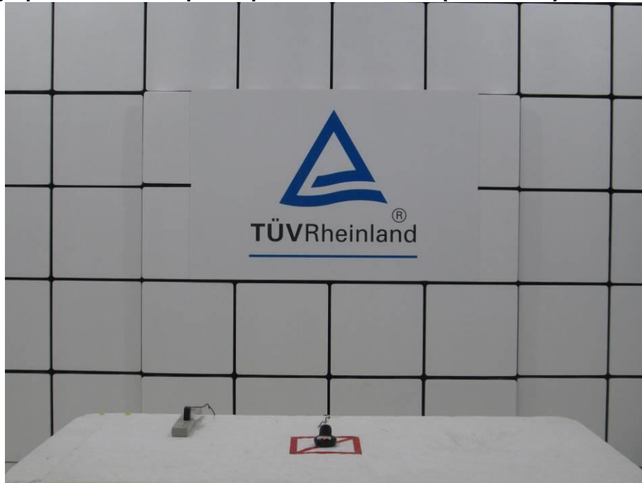
Photograph 19: Test Setup for Spurious Emissions (Front View)
