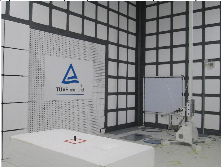
Photograph 13: Test Setup for Spurious Emissions (Back View 1)
