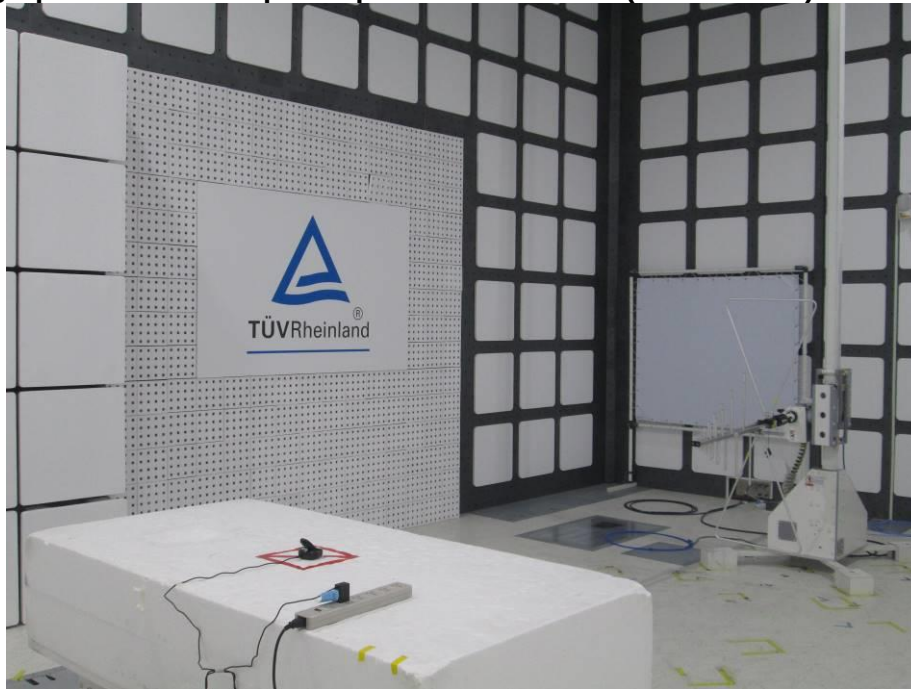
Photograph 21: Test Setup for Spurious Emissions (Back View 2)
