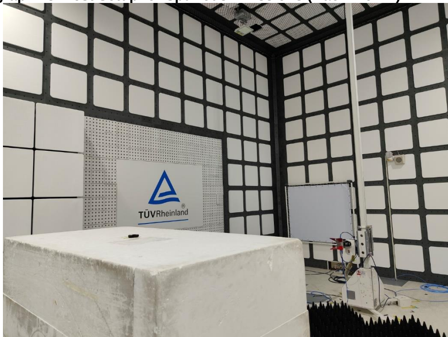
Photograph 18: Test Setup for Spurious Emissions (Back View 2)
