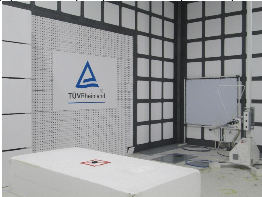
Photograph 17: Test Setup for Spurious Emissions (Back View 1)
