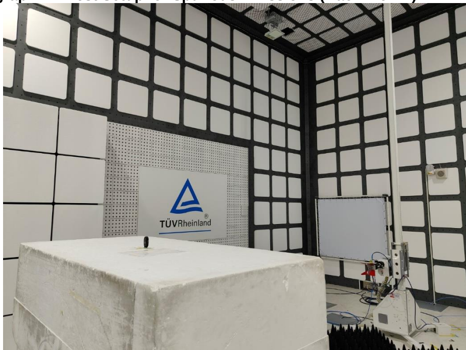
Photograph 14: Test Setup for Spurious Emissions (Back View 2)
