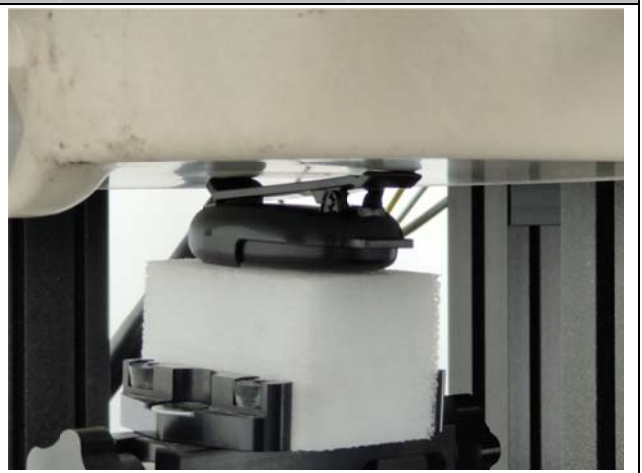
Back_0mm_Blet Clip
