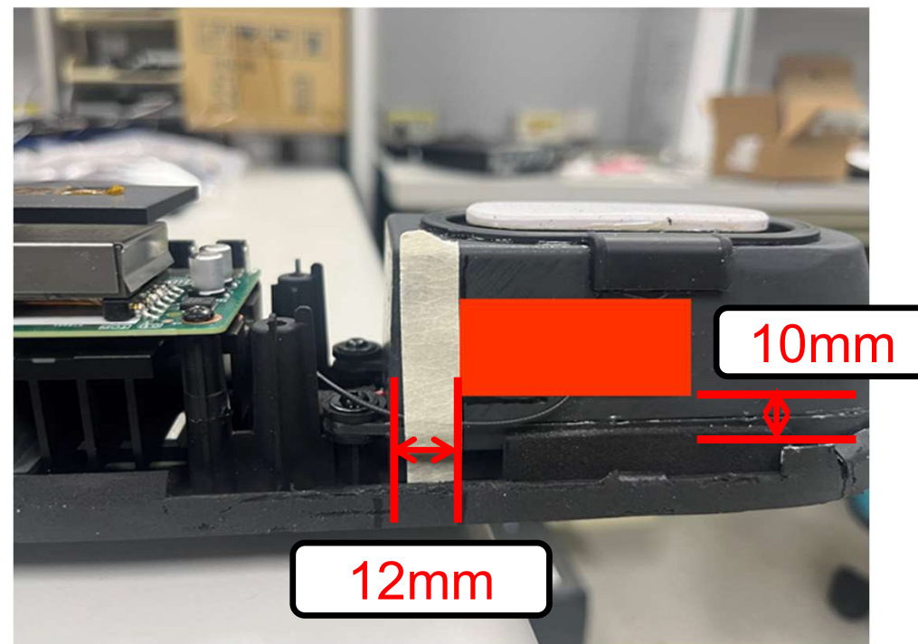
Aux Antenna
