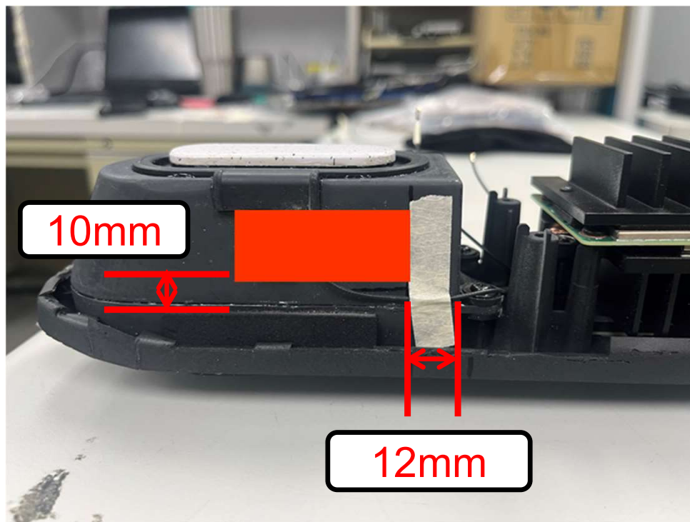
Main Antenna
