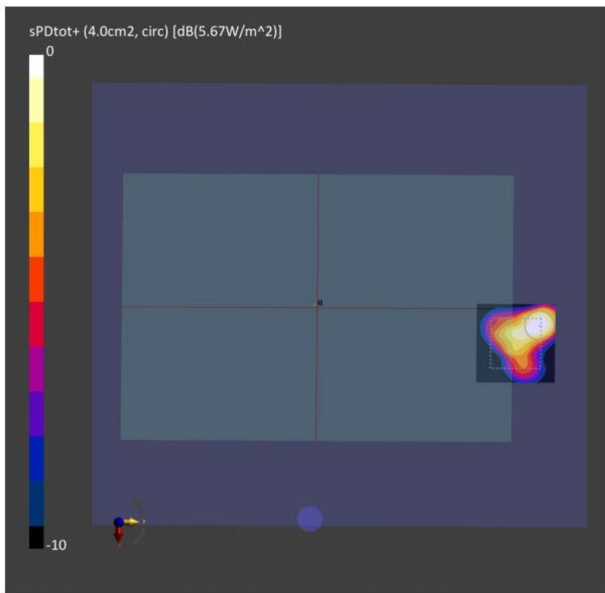
Figure 8-3: 4cm 2 -averaged power density distribution measured at input.power.limit of 5.67 dBm on the Bottom surface for n260 beam 30
