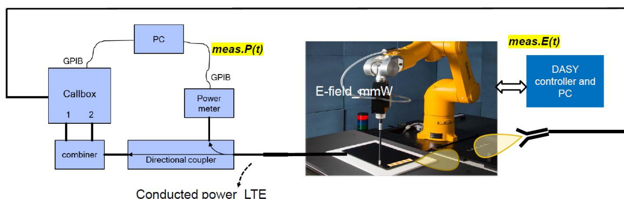
Figure 9-1 PD measurement setup
