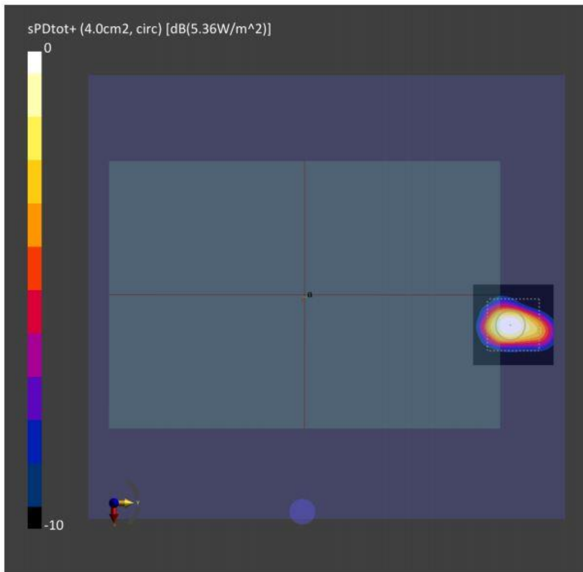
Figure 8-4: 4cm 2 -averaged power density distribution measured at input.power.limit of 5.36 dBm on the Right Side for n261 beam 29
