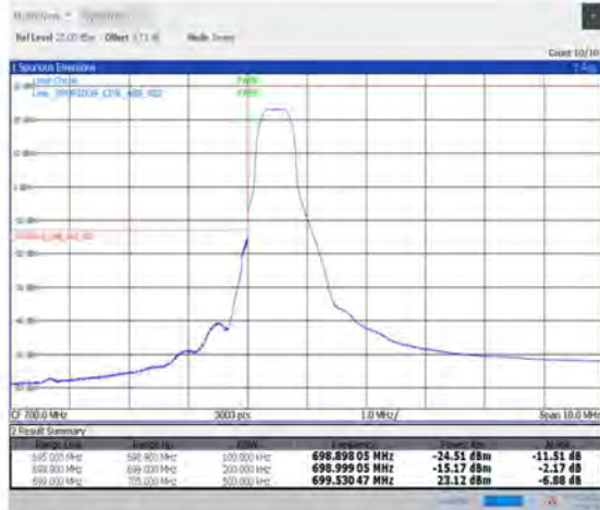
1-N12--15-15-L-1-DFT-PI2BPSK-Edge_1RB_Left-1@0-Ant1-PASS-see graph
