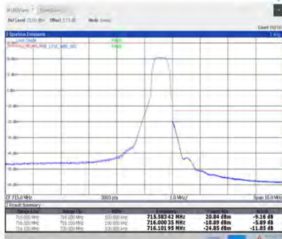
1-N12--15-10-H-5-CP-QPSK-Edge_1RB_Right-1@51-Ant1-PASS-see graph
