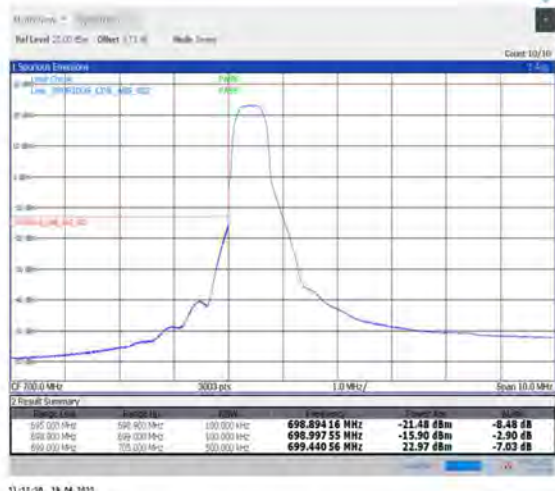
1-N12--15-10-L-1-DFT-PI2BPSK-Edge_1RB_Left-1@0-Ant1-PASS-see graph
