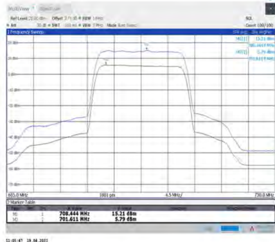
1-N12--15-15-M-2-CP-256QAM-Outer_Full-79@0- Ant1-9.42-100%-0.00-9.42-PASS-≤13
