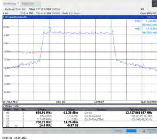
1-N12--15-15-L-3-DFT-16QAM-Outer_Full-75@0-Ant1-13.428-14.400-≤15-PASS
