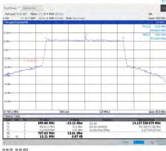
1-N12--15-15-M-8-CP-64QAM-Outer_Full-79@0-Ant1-14.158-15.210-≤15-PASS
