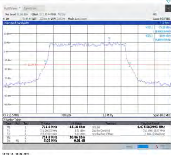
1-N12--15-5-H-5-DFT-256QAM-Outer_Full-25@0-Ant1-4.476-5.020-≤5-PASS
