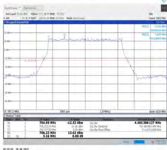
1-N12--15-5-M-2-DFT-PI2BPSK-Outer_Full-25@0-Ant1-4.485-5.160-≤5-PASS
