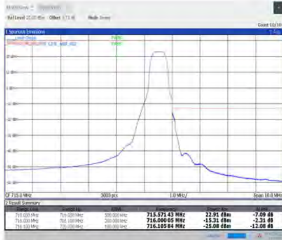
1-N12--15-15-H-2-DFT-PI2BPSK-Edge_1RB_Right-1@78-Ant1-PASS-see graph
