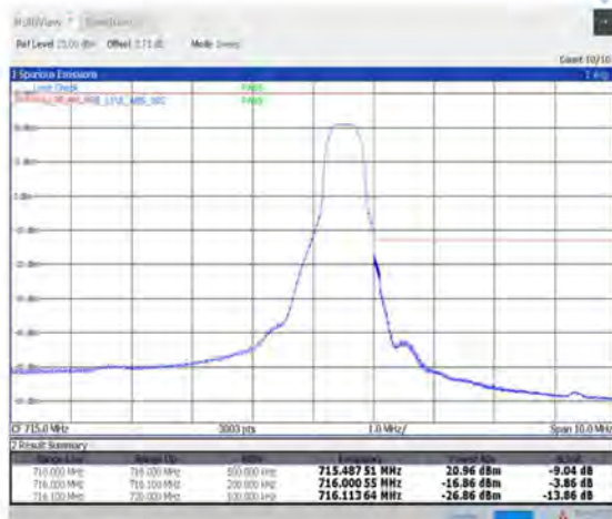
1-N12--15-15-H-5-CP-QPSK-Edge_1RB_Right-1@78-Ant1-PASS-see graph
