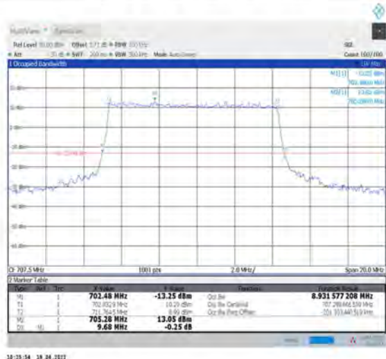
1-N12--15-10-M-3-DFT-16QAM-Outer_Full-50@0- Ant1-8.932-9.680-≤10-PASS
