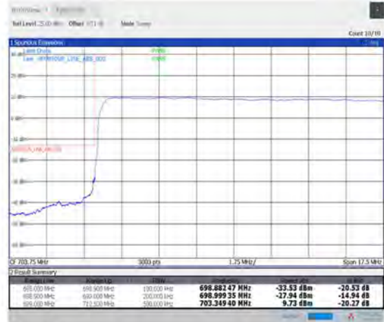
1-N12--15-15-L-3-DFT-PI2BPSK-Outer_Full-75@0-Ant1-PASS-see graph
