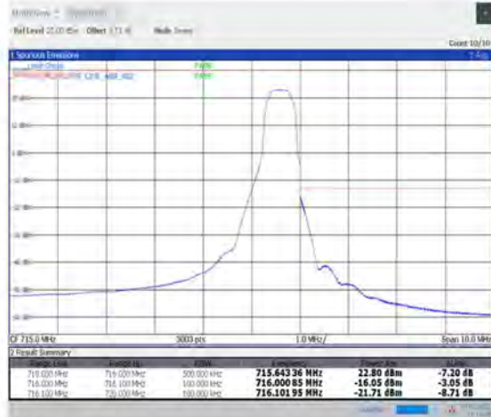
1-N12--15-10-H-2-DFT-PI2BPSK-Edge_1RB_Right-1@51-Ant1-PASS-see graph
