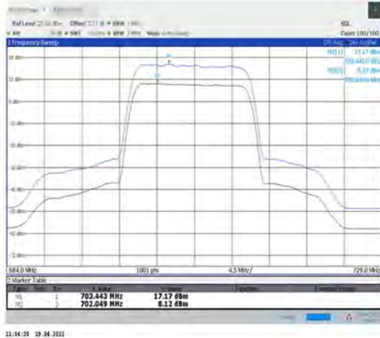
1-N12--15-15-L-1-DFT-256QAM-Outer_Full-75@0- Ant1-9.05-100%-0.00-9.05-PASS-≤13
