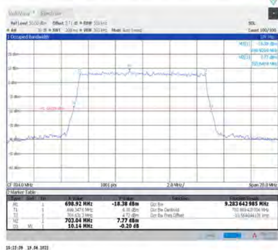
1-N12--15-10-L-9-CP-256QAM-Outer_Full-52@0-Ant1-9.284-10.140-≤10-PASS
