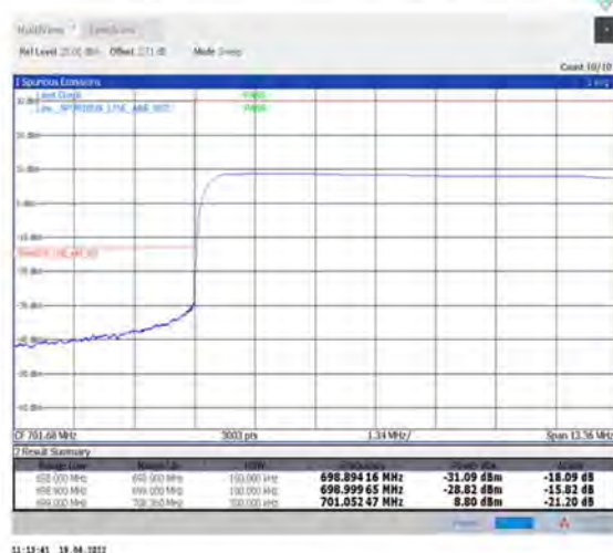
1-N12--15-10-L-6-CP-QPSK-Outer_Full-52@0-Ant1-PASS-see graph
