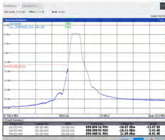
1-N12--15-15-L-4-CP-QPSK-Edge_1RB_Left-1@0-Ant1-PASS-see graph
