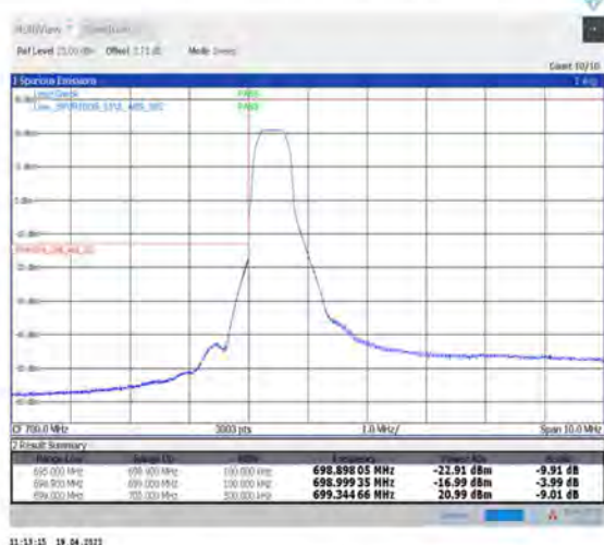
1-N12--15-10-L-4-CP-QPSK-Edge_1RB_Left-1@0-Ant1-PASS-see graph
