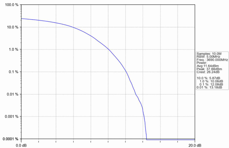
n48_30kHz_SISO_NTNV_20MHz_DFT-s-OFDM_16_QAM_3690MHz_Outer_Full
