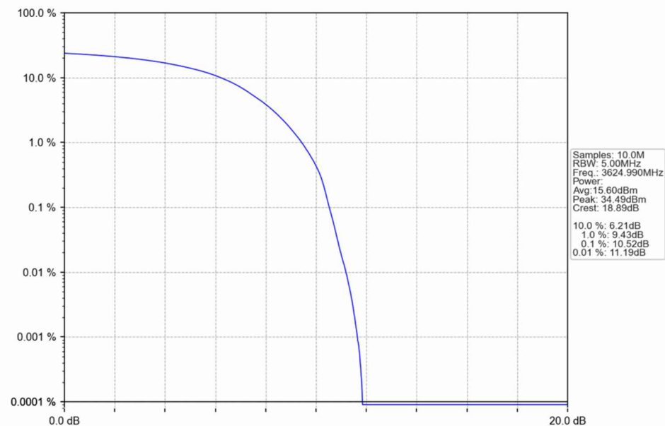
n48_30kHz_SISO_NTNV_10MHz_DFT-s-OFDM QPSK_3624.99MHz_Outer_Full
