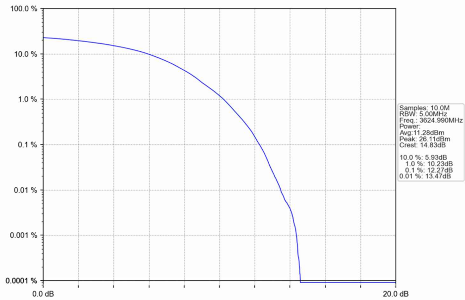
n48_30kHz_SISO_NTNV_20MHz_DFT-s-OFDM_16_QAM_3624.99MHz_Outer_Full
