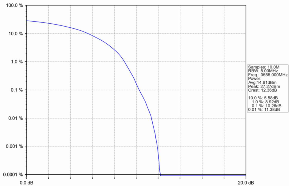
n48_30kHz_SISO_NTNV_10MHz_DFT-s-OFDM 16 QAM_3555MHz_Outer_Full
