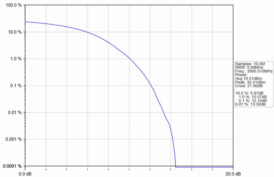
n48_30kHz_SISO_NTNV_20MHz_DFT-s-OFDM 16 QAM_3560.01MHz_Outer_Full
