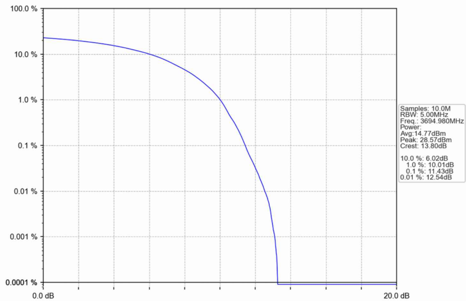
n48_30kHz_SISO_NTNV_10MHz_DFT-s-OFDM_16_QAM_3694.98MHz_Outer_Full
