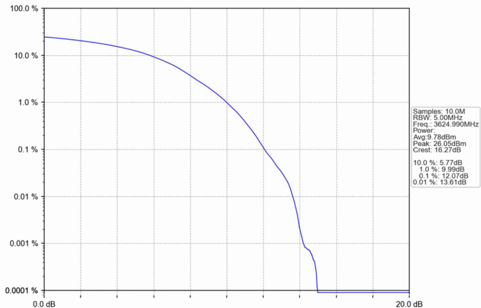
n48_30kHz_SISO_NTNV_40MHz_DFT-s-OFDM QPSK_3624.99MHz_Outer_Full
