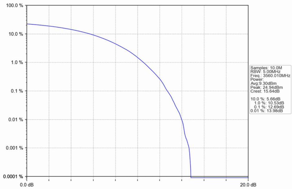
n48_30kHz_SISO_NTNV_20MHz_CP-OFDM 16 QAM_3560.01MHz_Outer_Full
