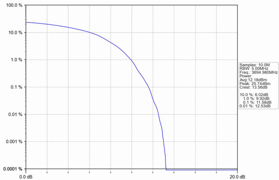
n48_30kHz_SISO_NTNV_10MHz_DFT-s-OFDM 256 QAM_3694.98MHz_Outer_Full
