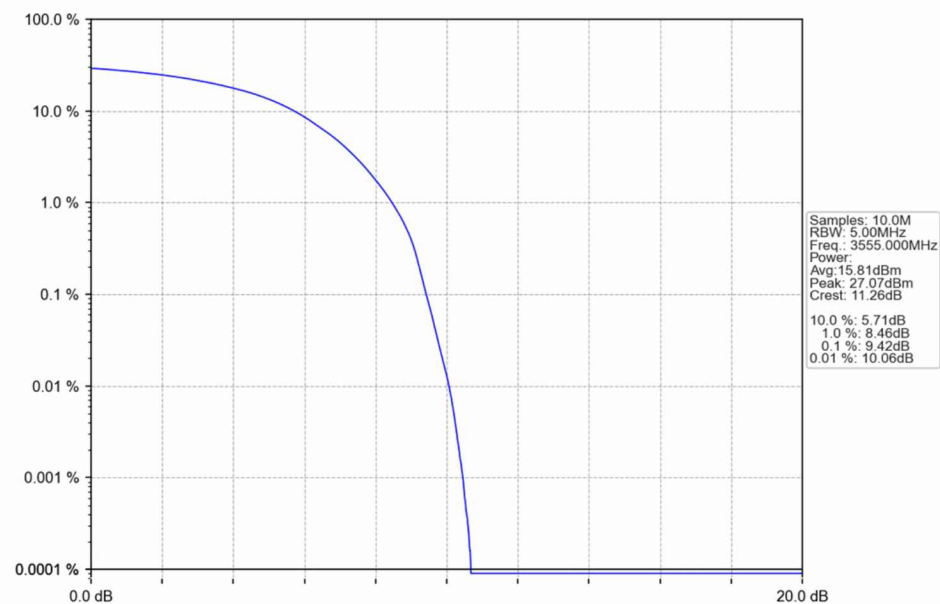
n48_30kHz_SISO_NTNV_10MHz_DFT-s-OFDM QPSK_3555MHz_Outer_Full
