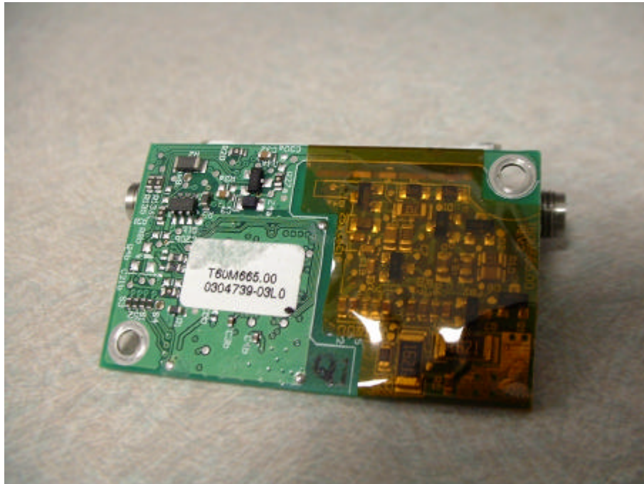
Bluetooth Transmitter card front side.
