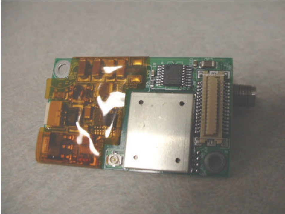
Bluetooth Transmitter card back side.
