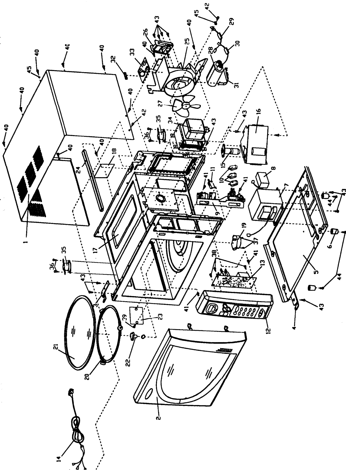
EXPLODE VIEWS MODEL: E7020X-Y
