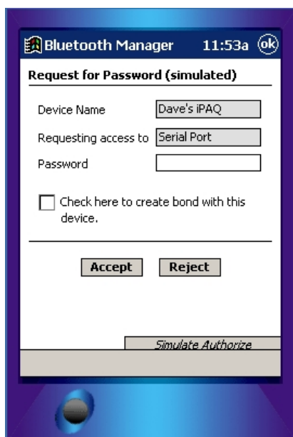
Figure 3-10. Authentication Dialogue
