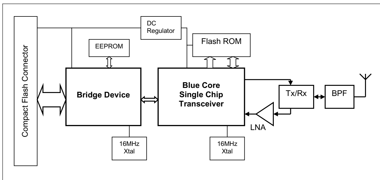
Figure 1: Block Diagram
