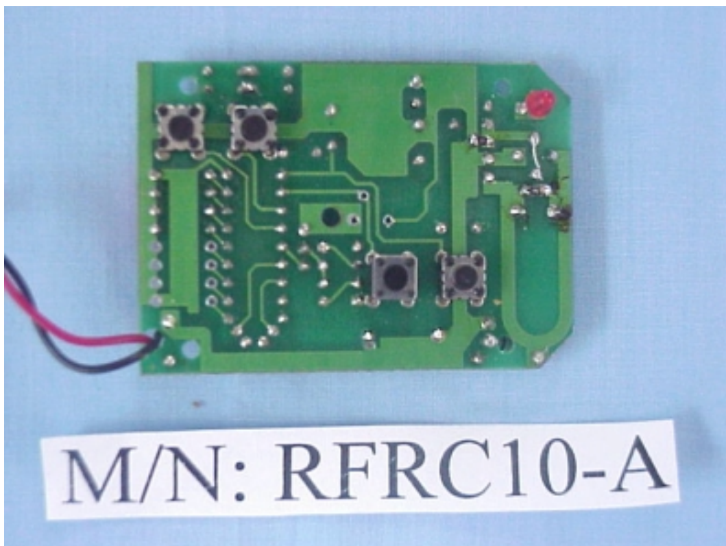
FIGURE 6 RADIO REMOTE CONTROLLER (M/N: RFRC10-A) SOLDERED SIDE
