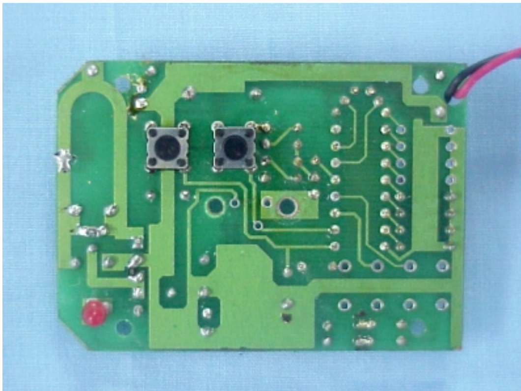
FIGURE 3 RADIO REMOTE CONTROLLER (M/N: ERX15-A) SOLDERED SIDE
