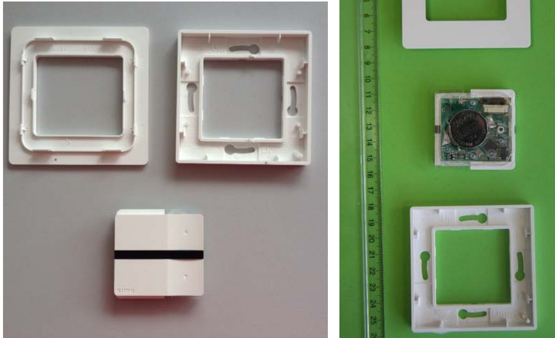
Figure 7.3.1 Front & Rear Internal View (1 Channel, 2008577)
