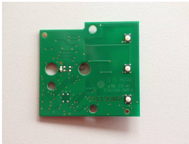
Figure 7.7 Foil Side (1 Channel, 2008577)
