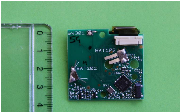
Figure 7.4 Component Side (5 Channel, 2008776)
