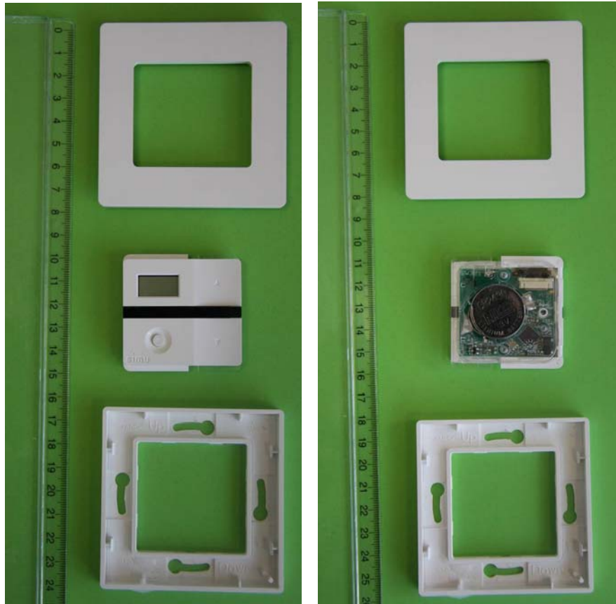
Figure 7.3 Front & Rear Internal View (5 Channel, 2008776)
