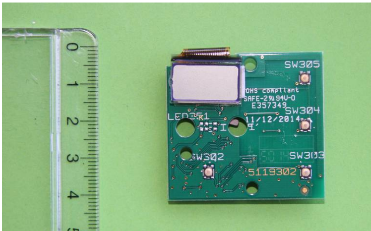
Figure 7.5 Foil Side (5 Channel, 2008776)
