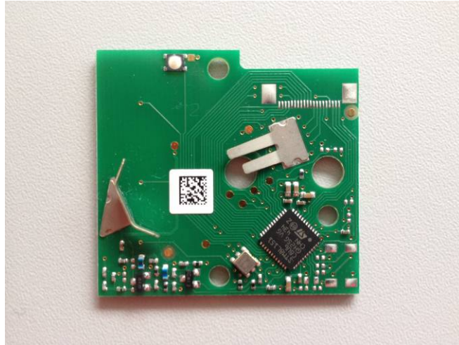
Figure 7.6 Component Side (1 Channel, 2008577)
