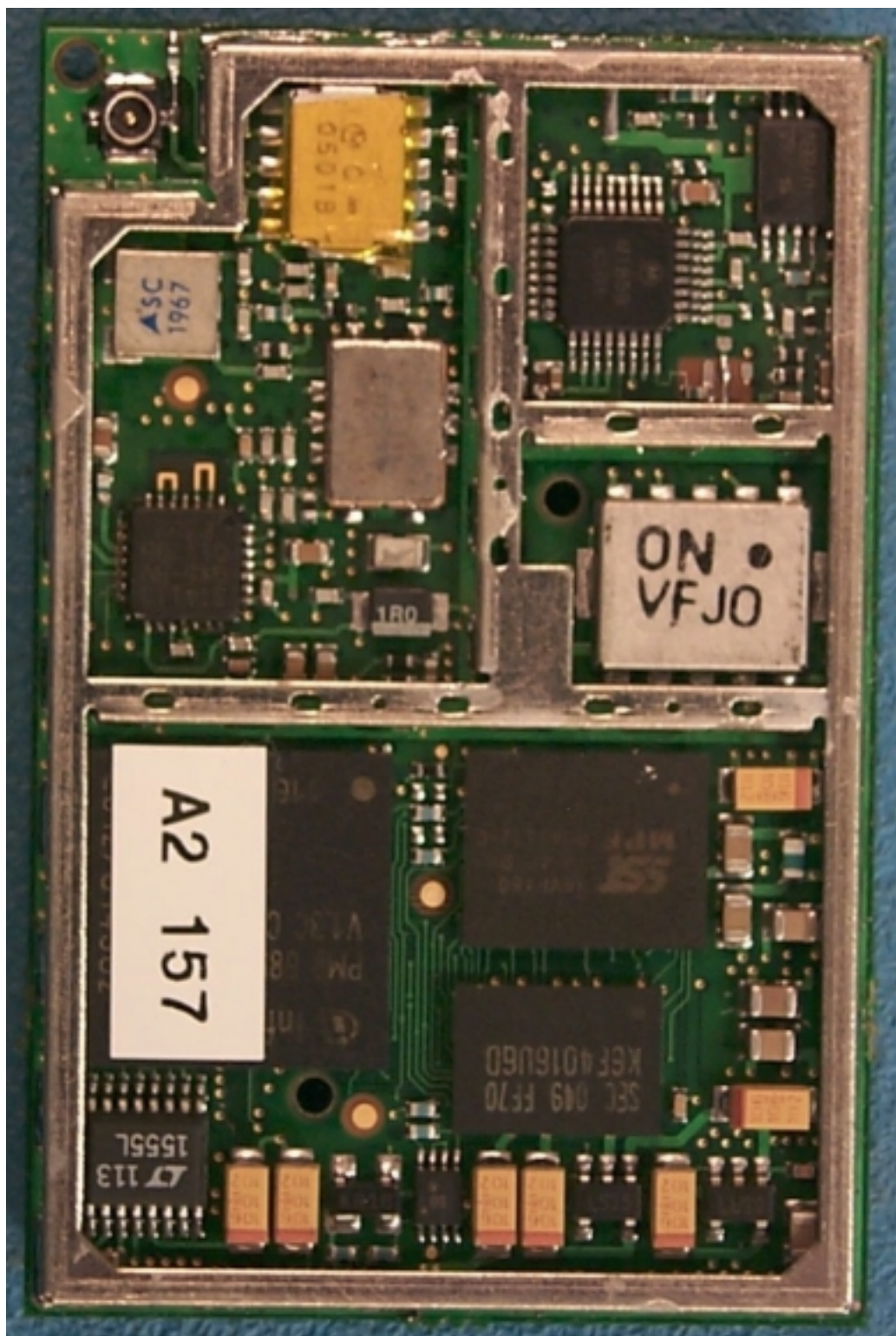
Photo 1. Top of Core Engine PCB (shields removed).
