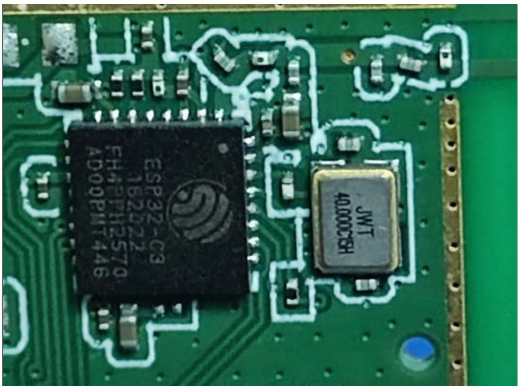
FIGURE 10 DIRECT CONNECT FULL COLOR A19 (M/N: CLEDA199CD1) CHIP&CRYSTAL ON BOARD
