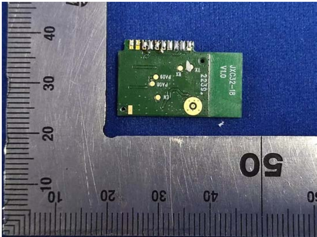
FIGURE 9 DIRECT CONNECT FULL COLOR A19 (M/N: CLEDA199CD1) RFBOARD BACK
