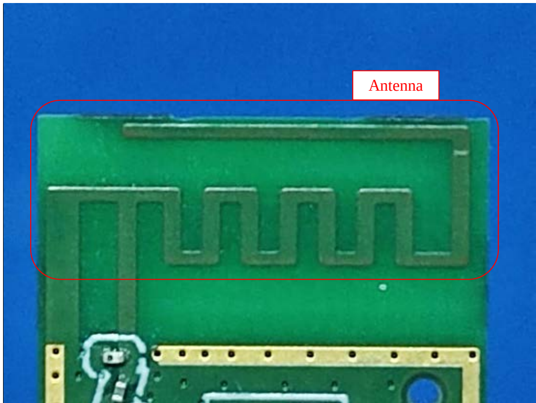
FIGURE 11 DIRECT CONNECT FULL COLOR A19 (M/N: CLEDA199CD1) ANTENNA
