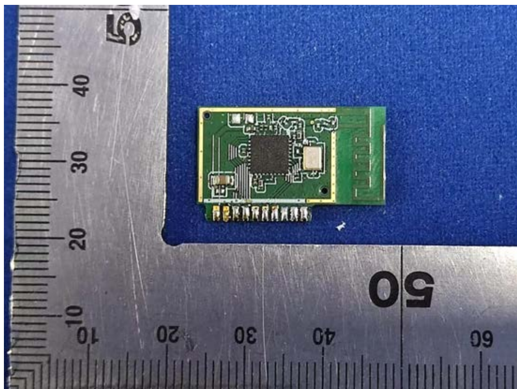
FIGURE 8 DIRECT CONNECT FULL COLOR A19 (M/N: CLEDA199CD1) RFBOARD FRONT
