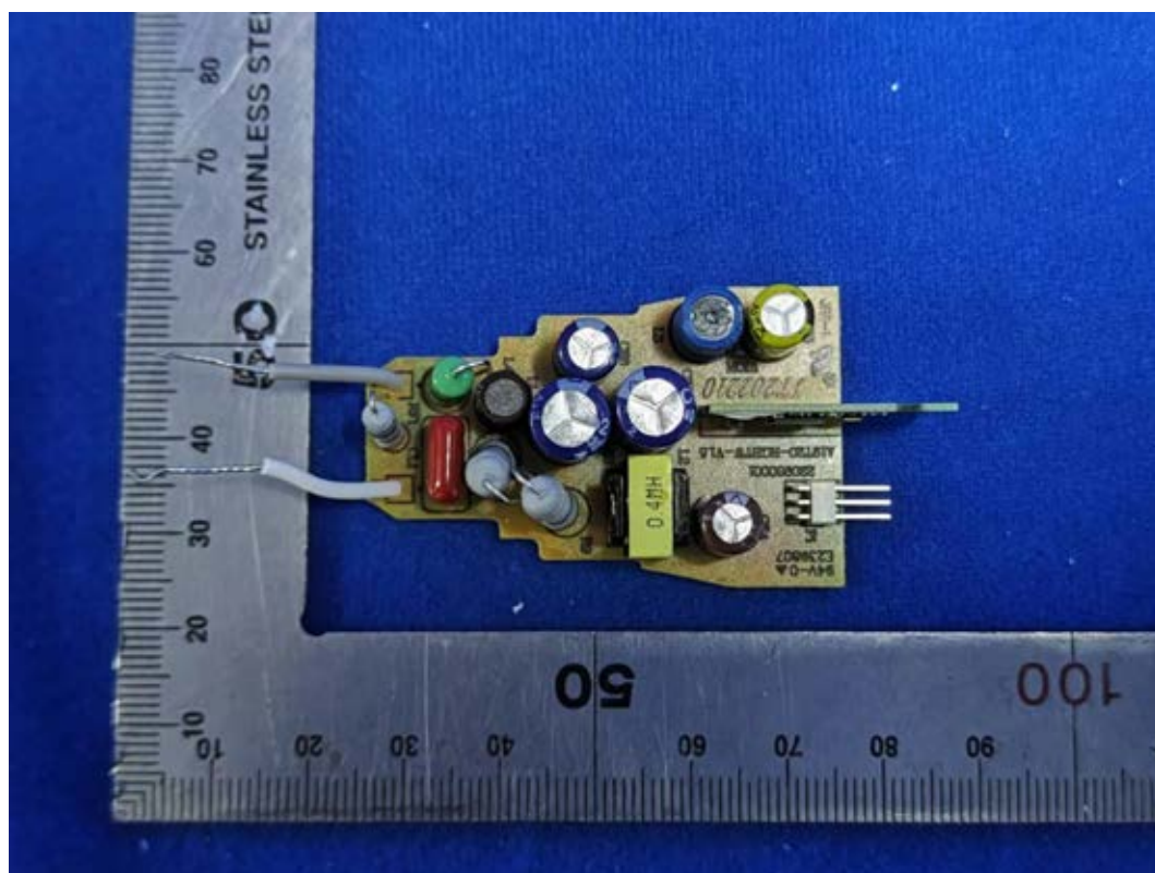
FIGURE 7 DIRECT CONNECT FULL COLOR A19 (M/N: CLEDA199CD1) MAINBOARD BACK
