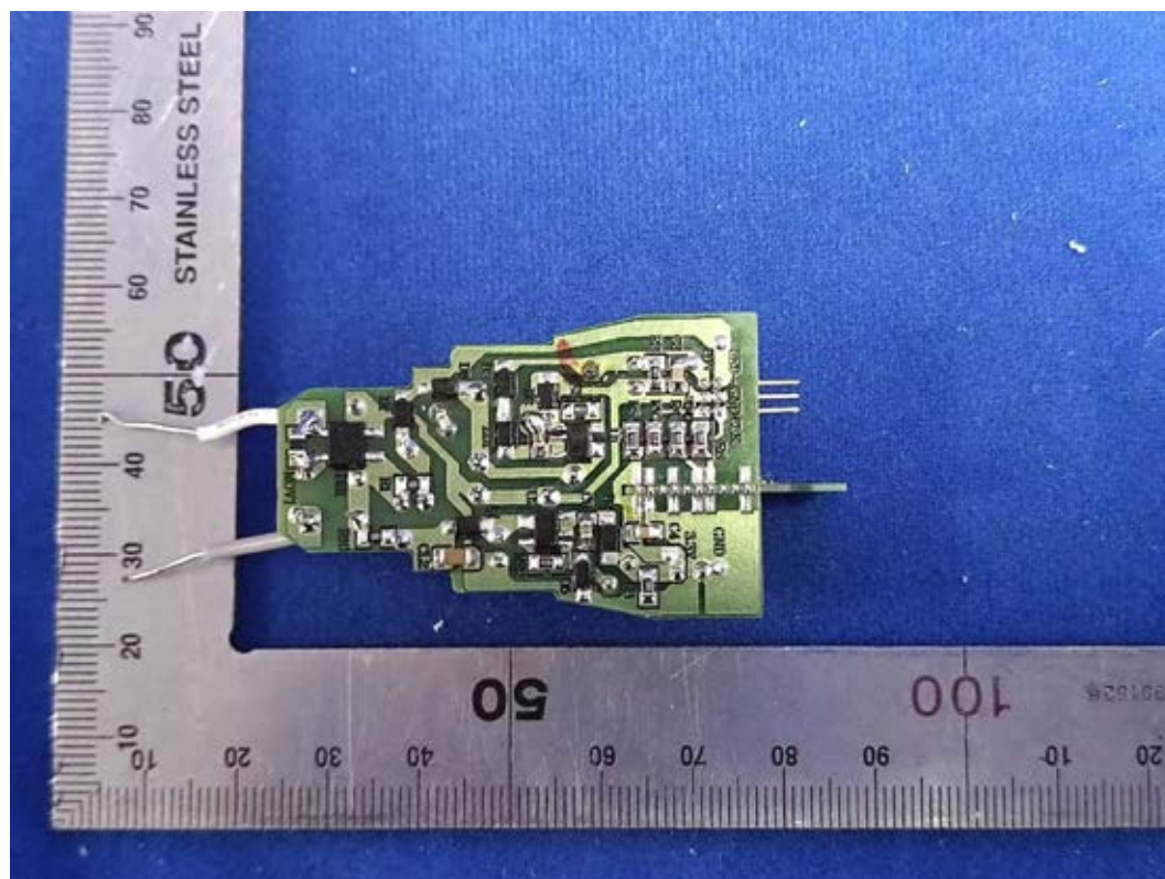
FIGURE 6 DIRECT CONNECT FULL COLOR A19 (M/N: CLEDA199CD1) MAINBOARD FRONT
