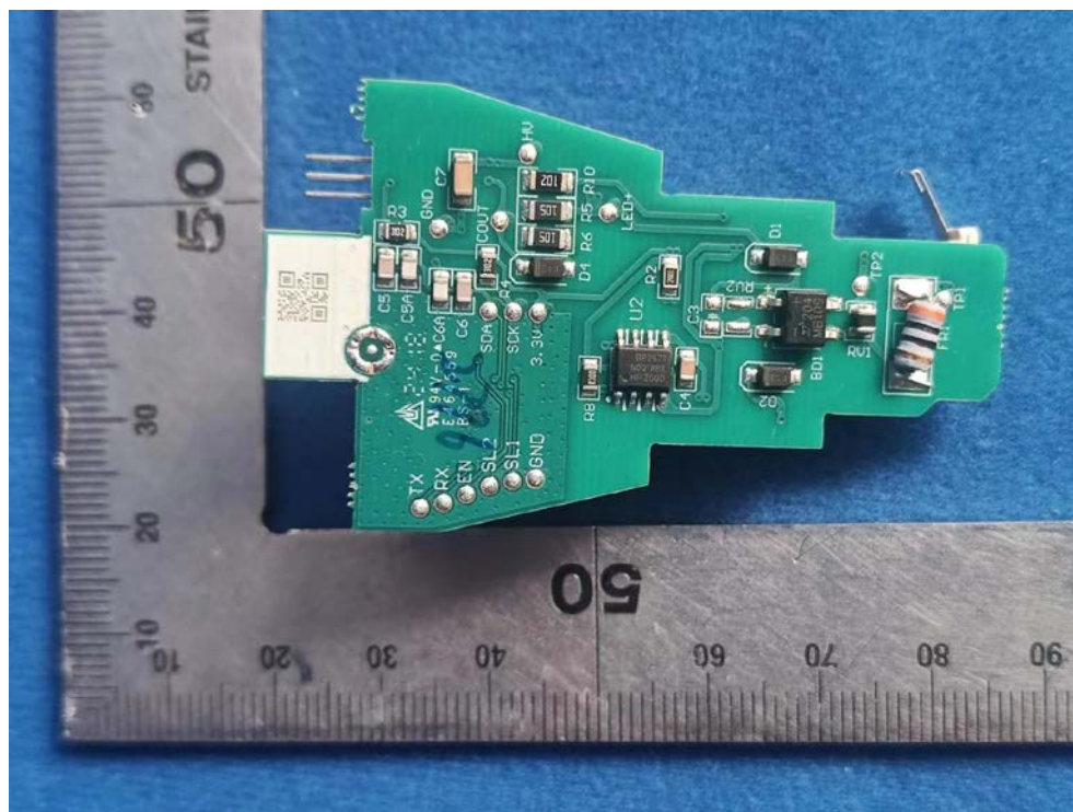
FIGURE 9 DIRECT CONNECT FULL COLOR A19 (CLEDA199CD1G) MAINBOARD BACK
