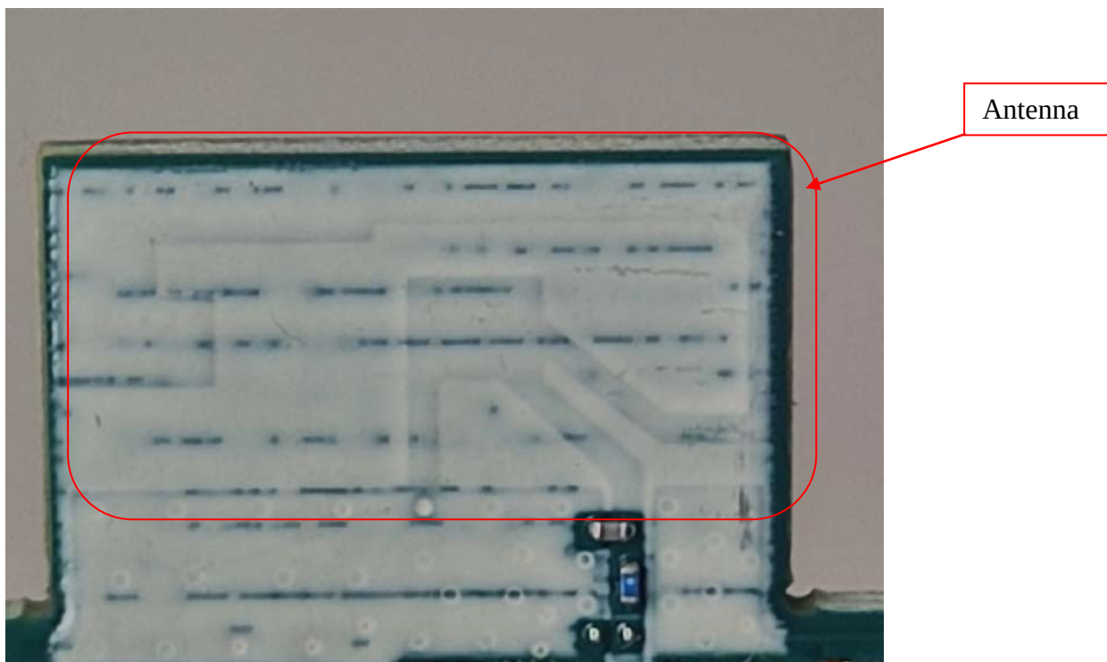
FIGURE 11 DIRECT CONNECT FULL COLOR A19 (CLEDA199CD1G) ANTENNA
