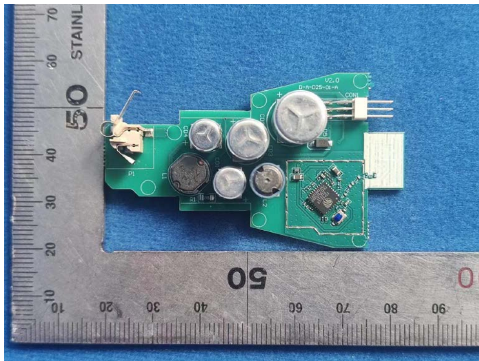
FIGURE 8 DIRECT CONNECT FULL COLOR A19 (CLEDA199CD1G) MAINBOARD FRONT
