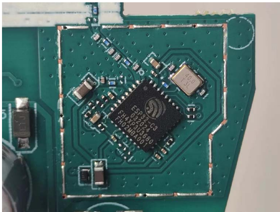
FIGURE 10 DIRECT CONNECT FULL COLOR A19 (CLEDA199CD1G) CHIP&CRYSTAL ON BOARD
