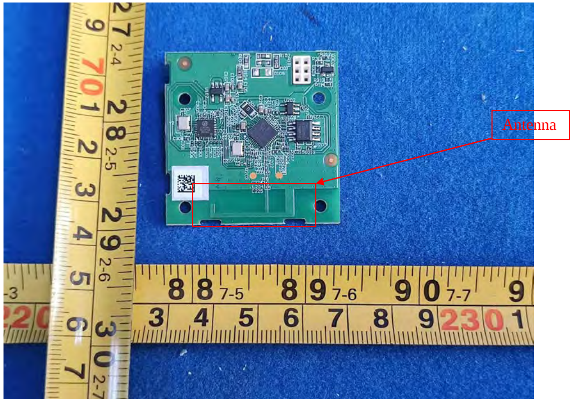
FIGURE 59 CYNIC DYNAMIC EFFECTS SMART CAFÉ LIGHTS (M/N: CCF72CDOD/ENS) RF BOARD BACK
