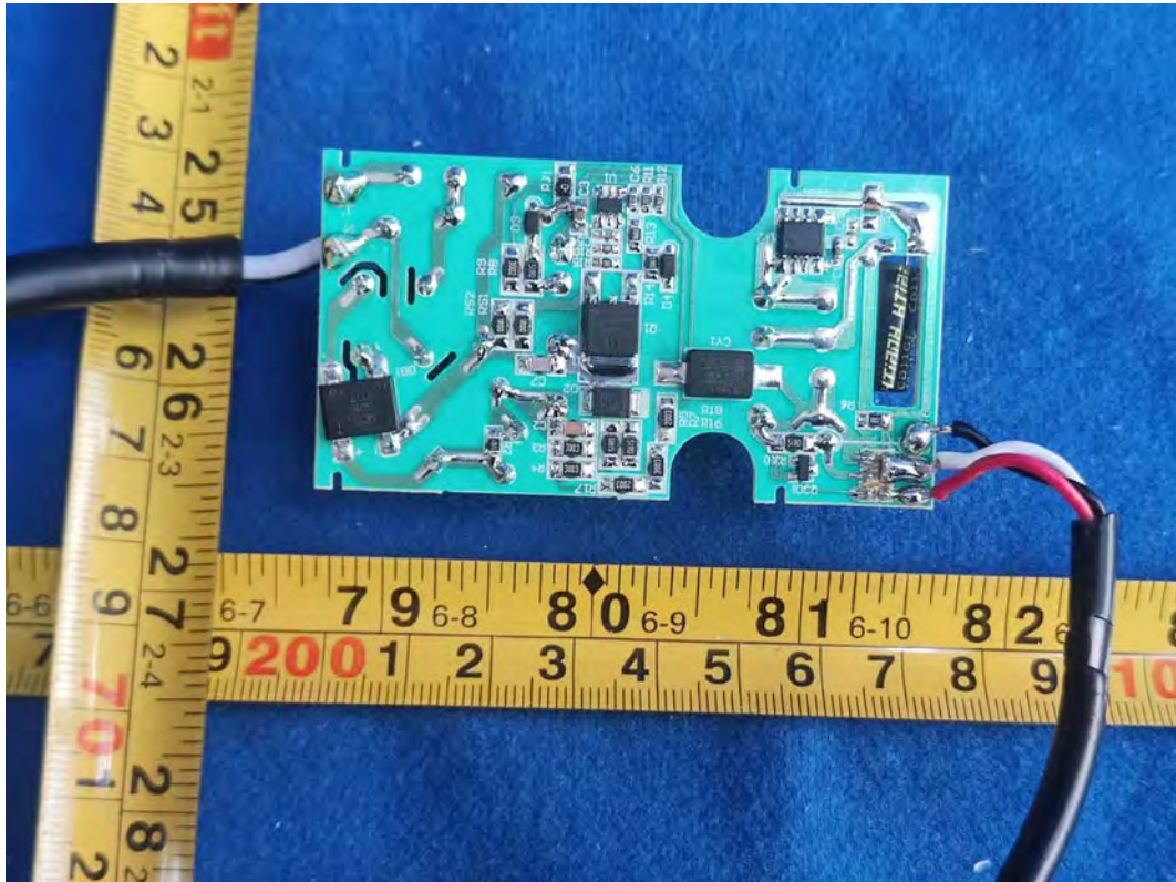
FIGURE 27 CYNIC DYNAMIC EFFECTS SMART CAFÉ LIGHTS (M/N: CCF24CDOD/ENS) MAINBOARD BACK
