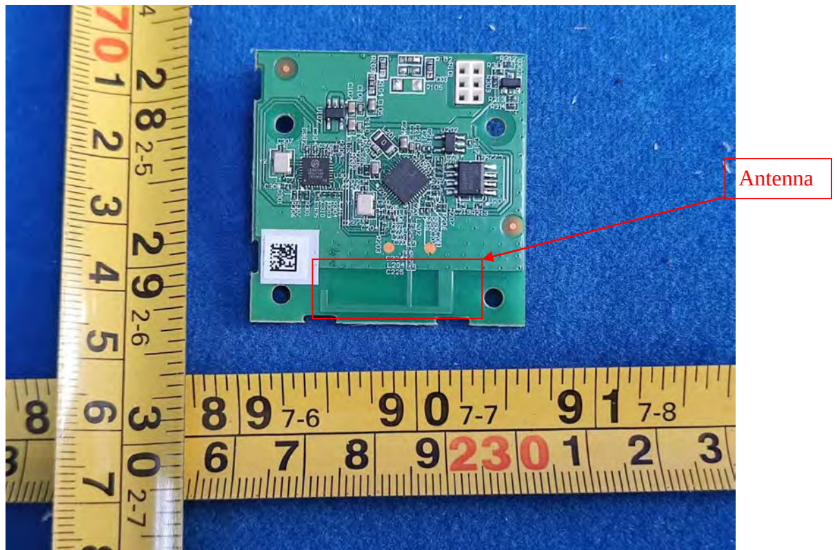
FIGURE 44 CYNCR DYNAMIC EFFECTS SMART CAFÉ LIGHTS (M/N: CCF96CDOD/ENS) RF BOARD BACK
