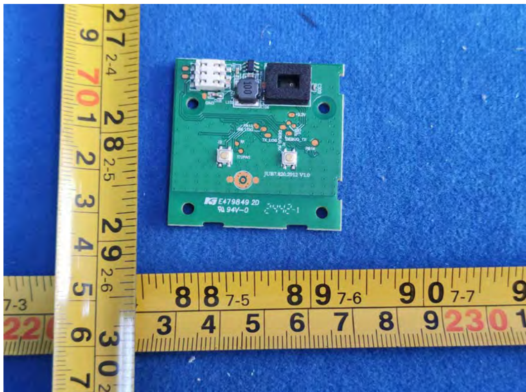
FIGURE 59 CYNIC DYNAMIC EFFECTS SMART CAFÉ LIGHTS (M/N: CCF72CDOD/ENS) RF BOARD BACK
