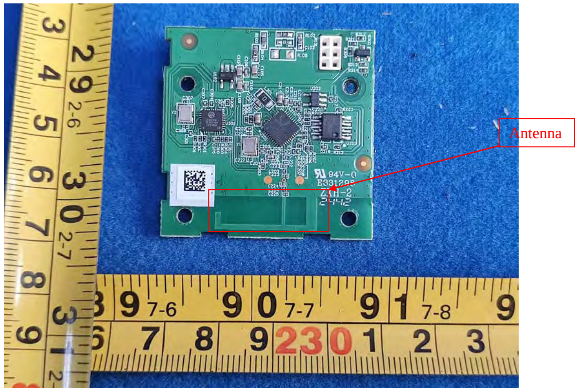
FIGURE 29 CYNCR DYNAMIC EFFECTS SMART CAFÉ LIGHTS (M/N: CCF24CDOD/ENS) RF BOARD BACK
