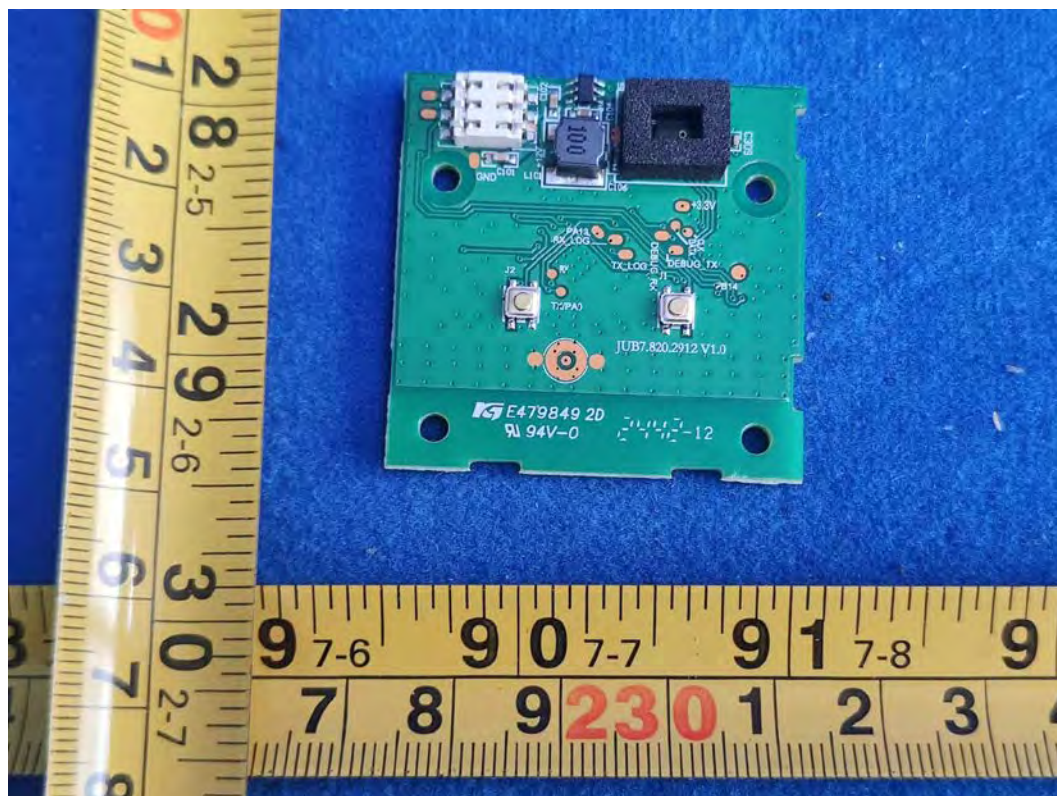
FIGURE 14 CYNCR DYNAMIC EFFECTS SMART CAFÉ LIGHTS (M/N: CCF48CDOD/ENS) RF BOARD BACK
