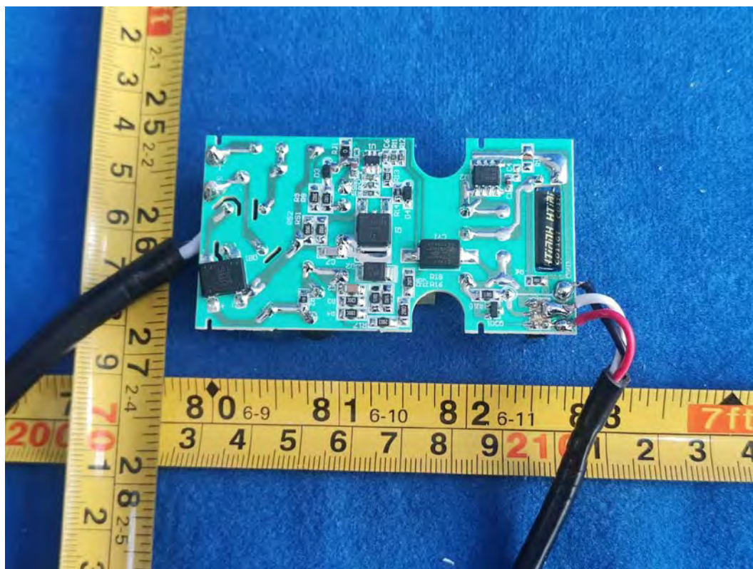
FIGURE 12 CYNIC DYNAMIC EFFECTS SMART CAFÉ LIGHTS (M/N: CCF48CDOD/ENS) MAINBOARD BACK
