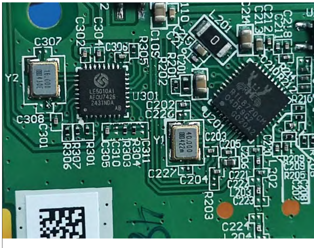
FIGURE 15 CYNIC DYNAMIC EFFECTS SMART CAFÉ LIGHTS (M/N: CCF48CDOD/ENS) CHIP&CRYSTAL ON BOARD
