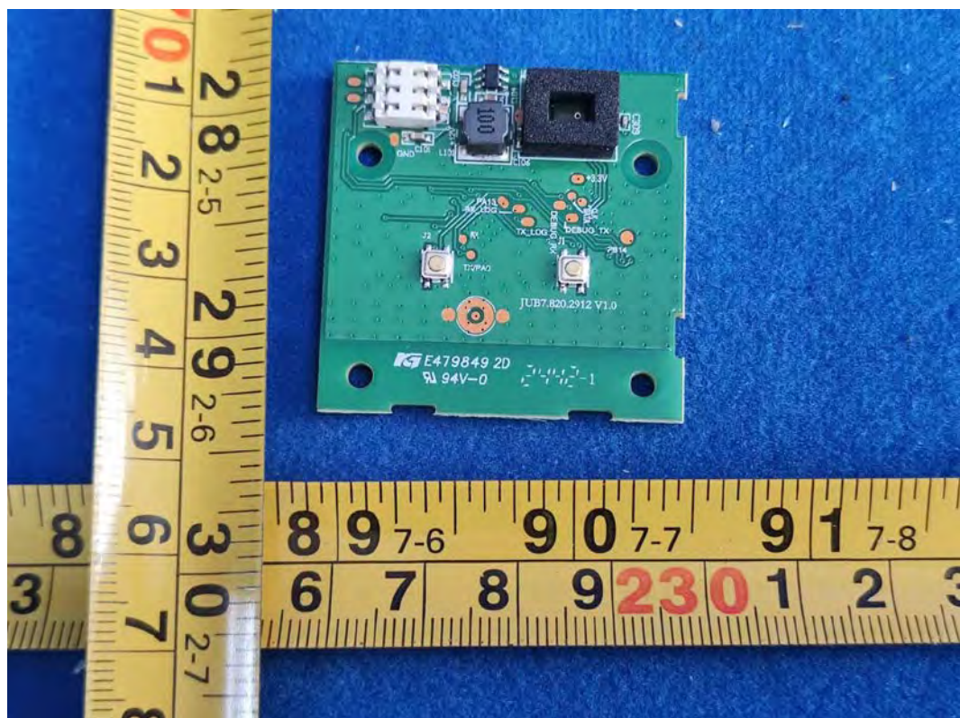
FIGURE 44 CYNCR DYNAMIC EFFECTS SMART CAFÉ LIGHTS (M/N: CCF96CDOD/ENS) RF BOARD BACK
