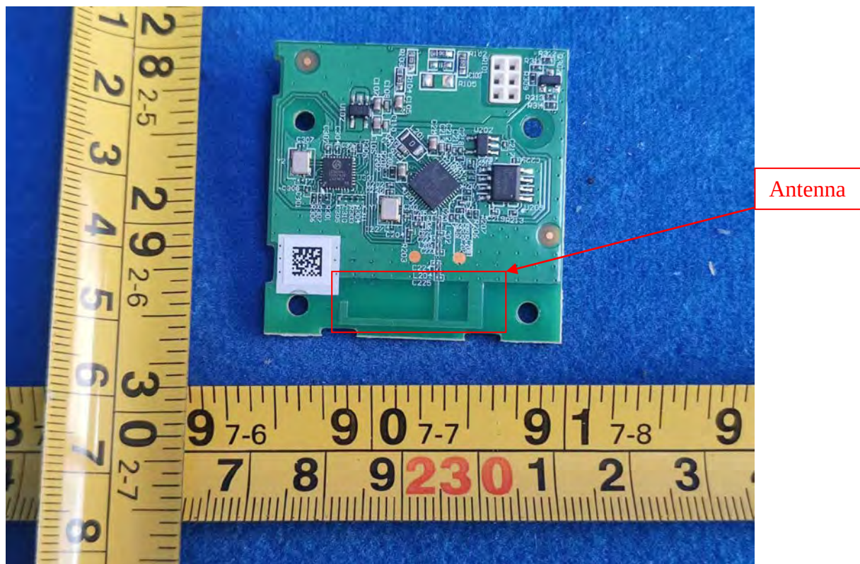
FIGURE 14 CYNCR DYNAMIC EFFECTS SMART CAFÉ LIGHTS (M/N: CCF48CDOD/ENS) RF BOARD BACK
