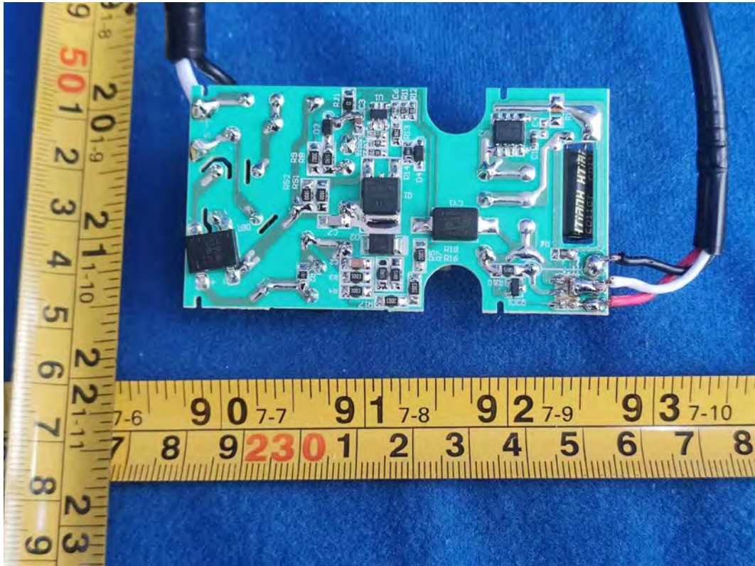
FIGURE 57 CYNIC DYNAMIC EFFECTS SMART CAFÉ LIGHTS (M/N: CCF72CDOD/ENS) MAINBOARD BACK
