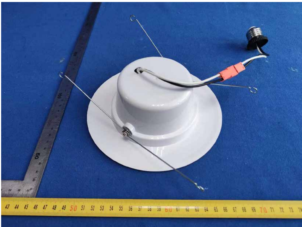
FIGURE 2 DOWNLIGHT (CFIXRSCR6CRVD) BACK APPEARANCE
