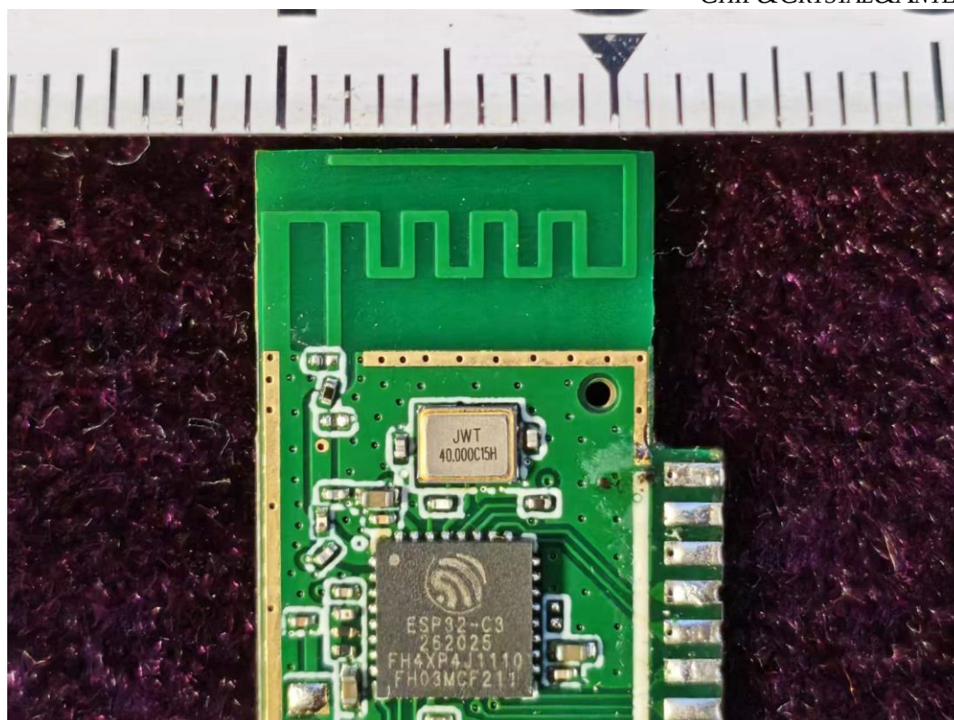
FIGURE 14 CYNC SHOPLIGHT (M/N: CFIXSHP46CDMAT) CHIP&CRYSTAL&ANTENNA
