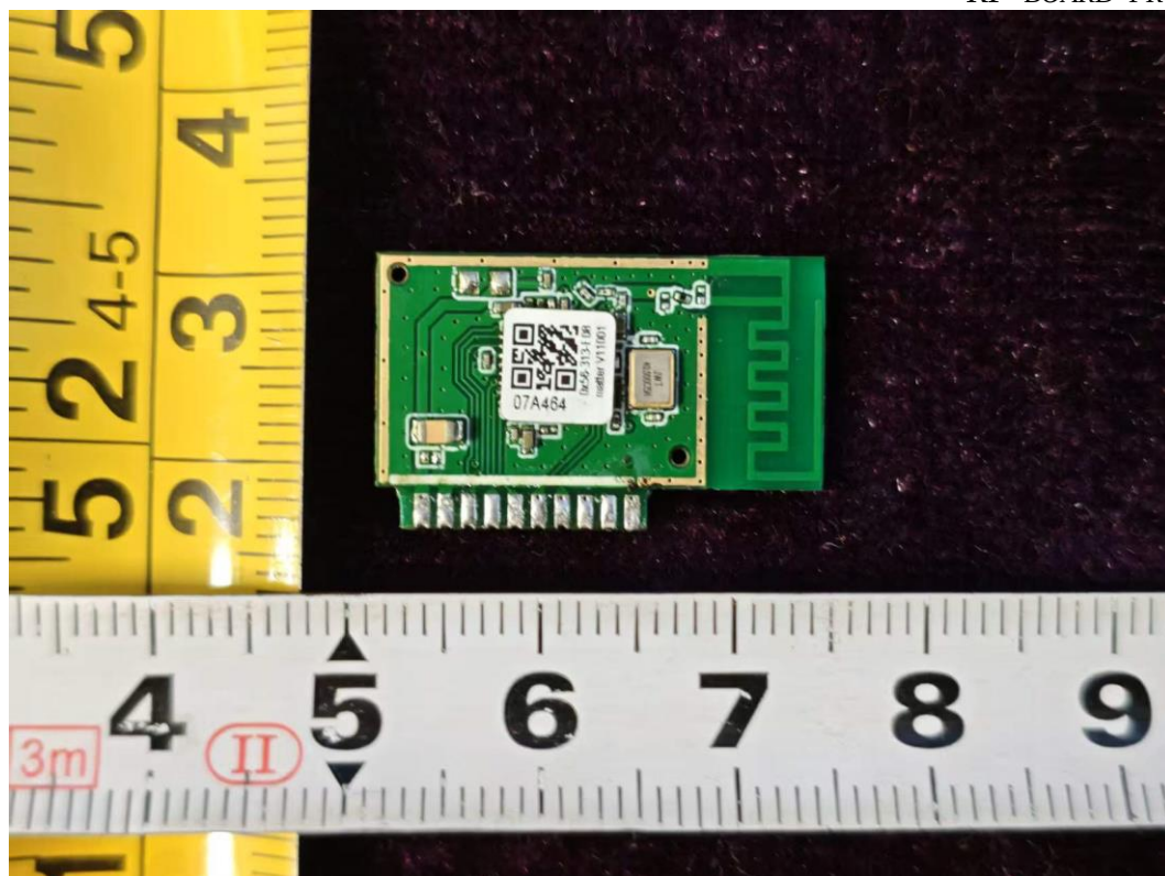
FIGURE 12 CYNC SHOPLIGHT (M/N: CFIXSHP46CDMAT) RF BOARD FRONT
