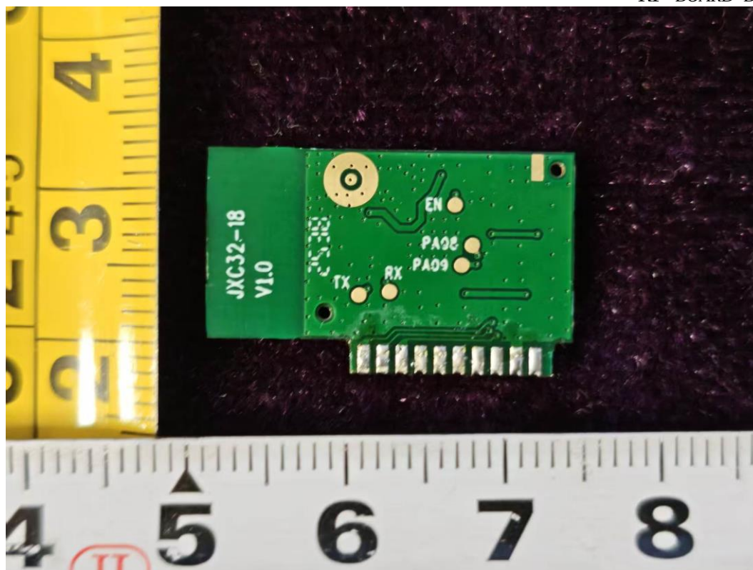
FIGURE 13 CYNC SHOPLIGHT (M/N: CFIXSHP46CDMAT) RF BOARD BACK
