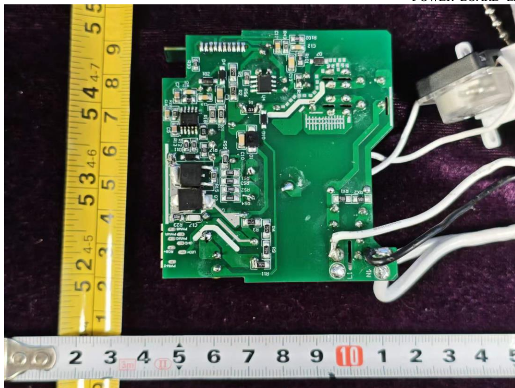
FIGURE 11 CYNC SHOPLIGHT (M/N: CFIXSHP46CDMAT) POWER BOARD BACK
