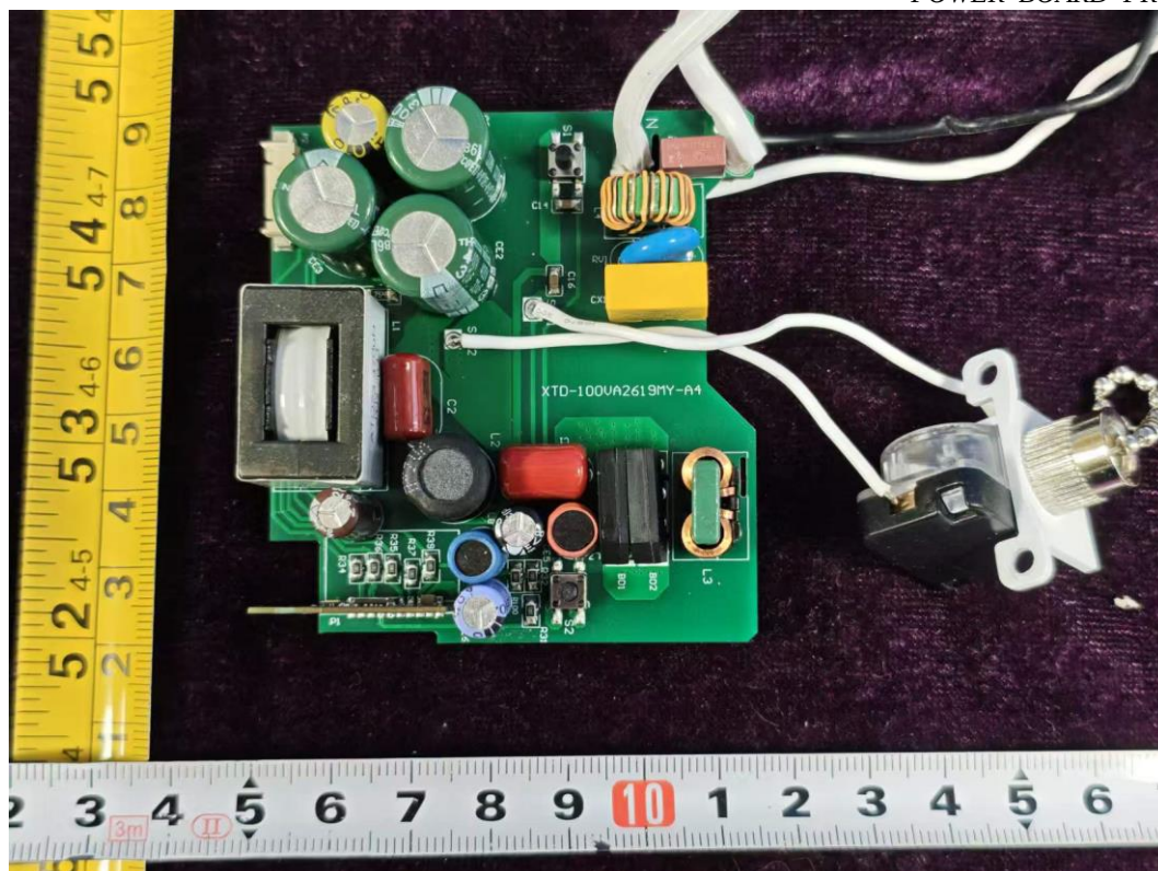
FIGURE 10 CYNC SHOPLIGHT (M/N: CFIXSHP46CDMAT) POWER BOARD FRONT
