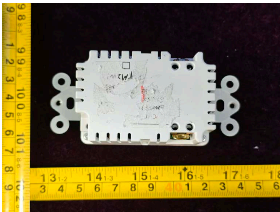
FIGURE 6 IN-WALL OUTLET (M/N: COTLSTD2PM2W1) OUT-6
