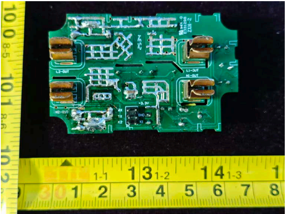
FIGURE 9 IN-WALL OUTLET (M/N: COTLSTD2PM2W1) BOARD1-2
