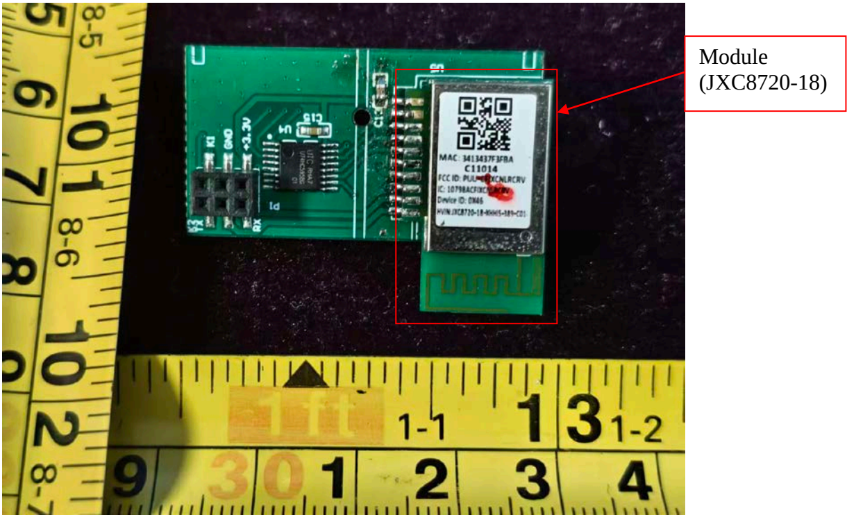
FIGURE 11 IN-WALL OUTLET (M/N: COTLSTD2PM2W1) BOARD2-2
