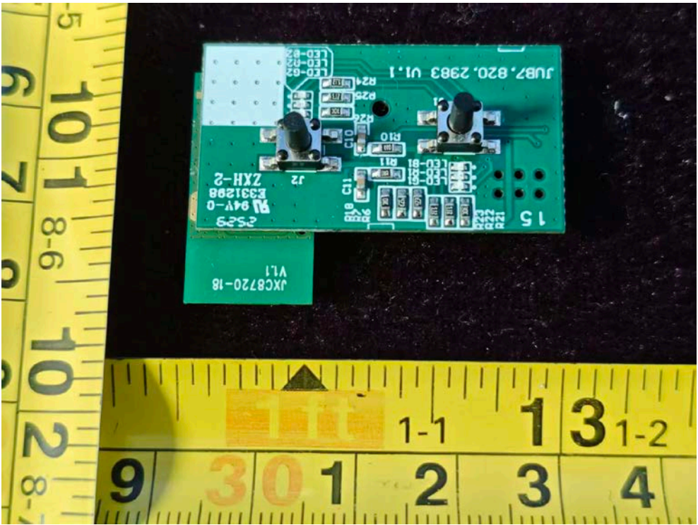
FIGURE 10 IN-WALL OUTLET (M/N: COTLSTD2PM2W1) BOARD2-1
