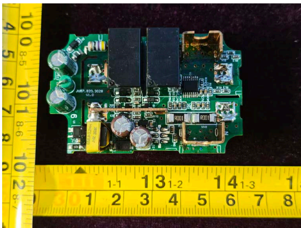
FIGURE 8 IN-WALL OUTLET (M/N: COTLSTD2PM2W1) BOARD1-1
