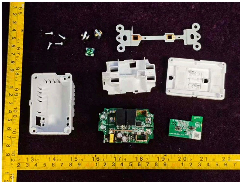
FIGURE 7 IN-WALL OUTLET (M/N: COTLSTD2PM2W1) COVER REMOVED
