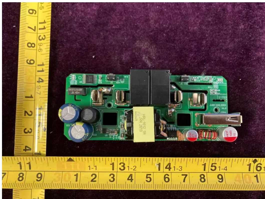
FIGURE 9 DUAL SOCKETS INDOOR PLUG (M/N: CPLGID2BLW1MS) POWER BOARD FRONT
