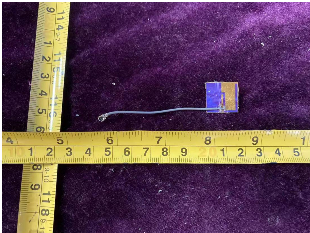
FIGURE 17 DUAL SOCKETS INDOOR PLUG (M/N: CPLGID2BLW1MS) ANTENNA1 FRONT
