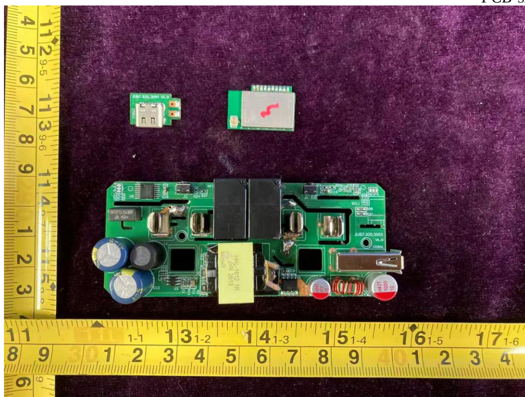
FIGURE 8 DUAL SOCKETS INDOOR PLUG (M/N: CPLGID2BLW1MS) PCB SPLIT
