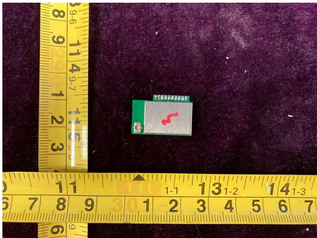
FIGURE 13 DUAL SOCKETS INDOOR PLUG (M/N: CPLGID2BLW1MS) RF BOARD FRONT
