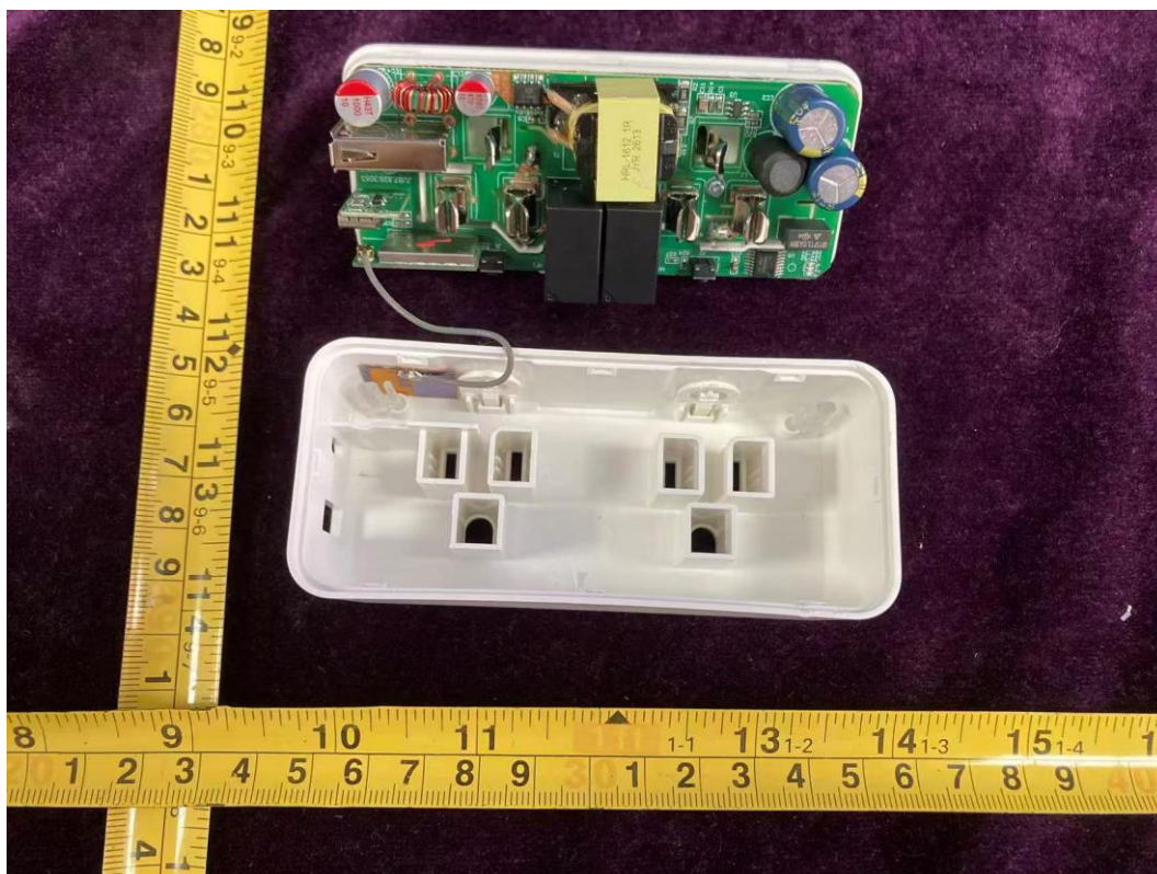
FIGURE 7 DUAL SOCKETS INDOOR PLUG (M/N: CPLGID2BLW1MS) COVER REMOVED
