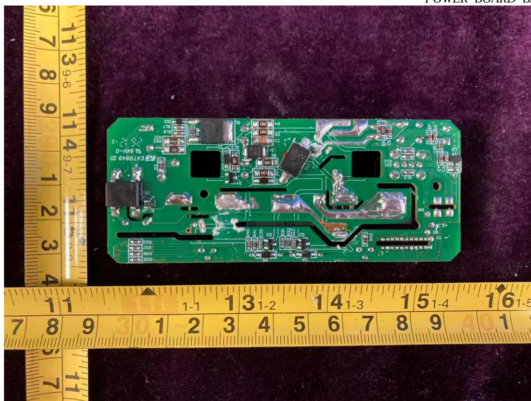
FIGURE 10 DUAL SOCKETS INDOOR PLUG (M/N: CPLGID2BLW1MS) POWER BOARD BACK
