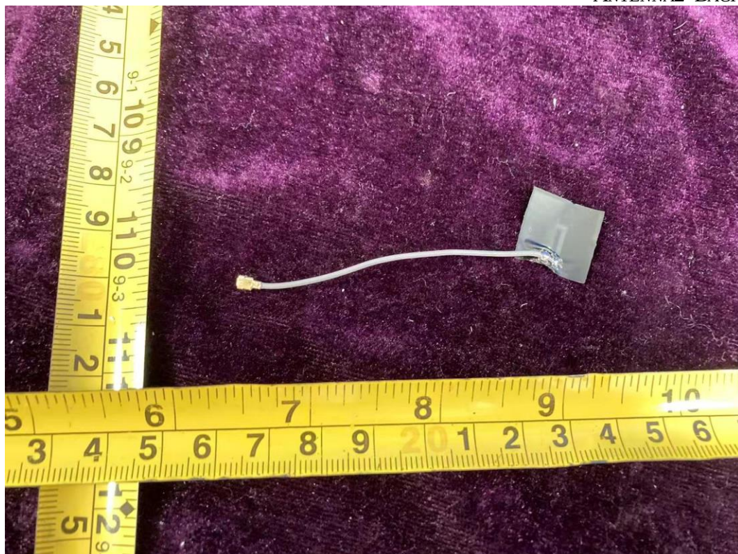
FIGURE 20 DUAL SOCKETS INDOOR PLUG (M/N: CPLGID2BLW1MS) ANTENNA2 BACK
