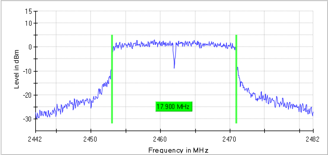
Mode 1 / CH11 (2462MHz) 6 dB Bandwidth
