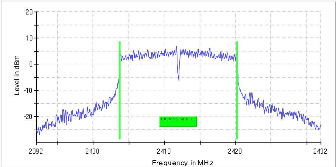
6dB Occupied Bandwidth Mode 1 / CH1 (2412MHz)
