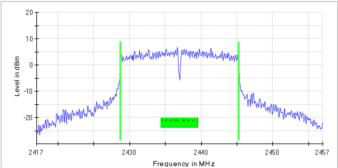
Mode 1 / CH6 (2437MHz)
