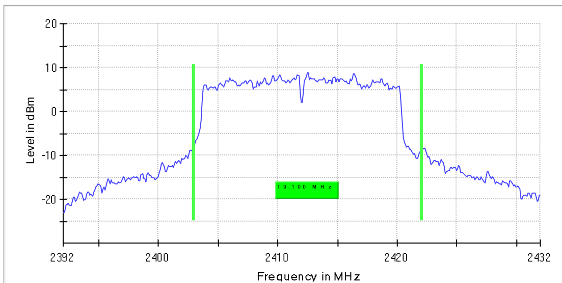
99% Occupied Bandwidth Mode 1 / CH1 (2412 MHz)
