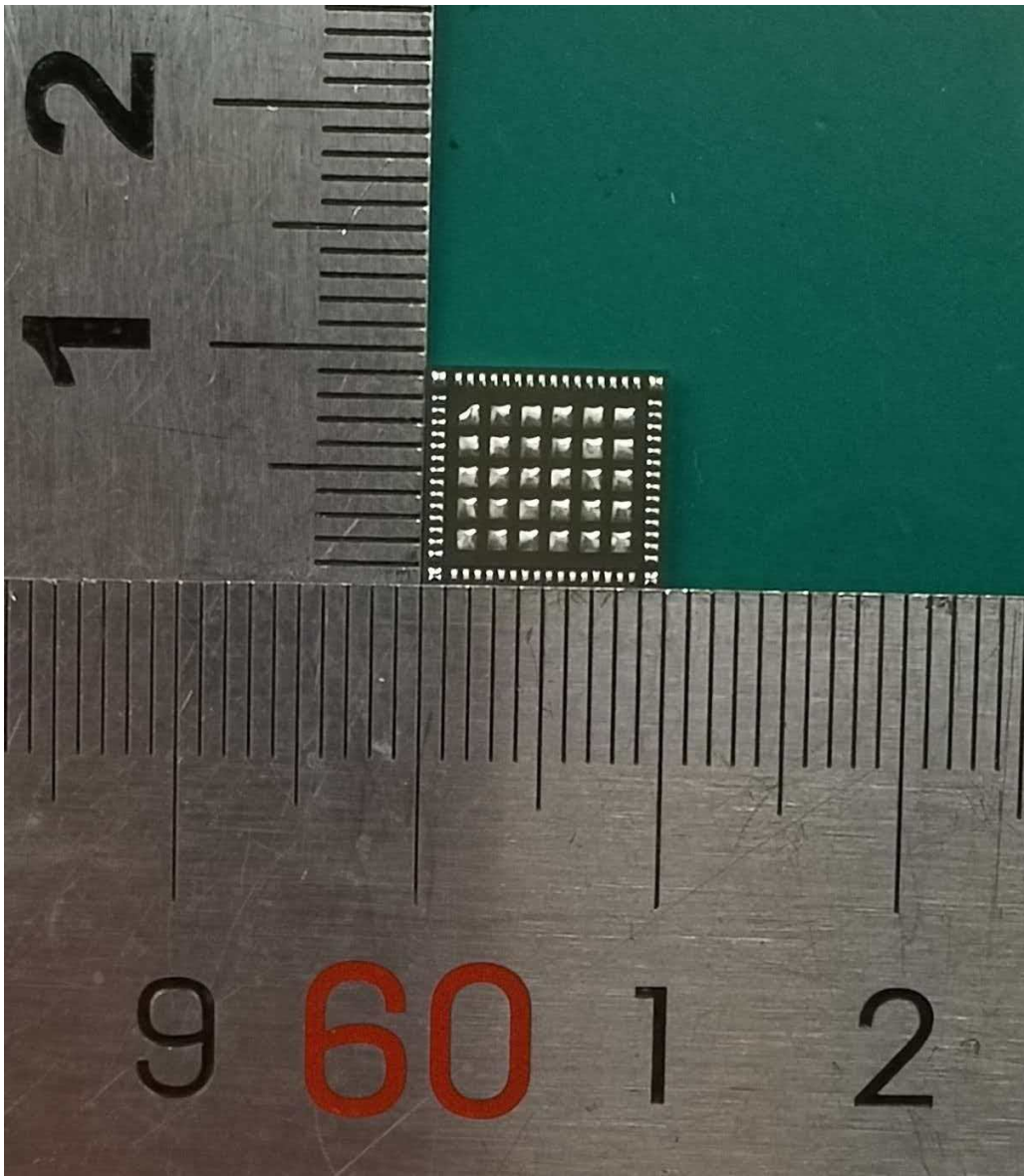
FIGURE 2 WiFi AND BLUETOOTH MODULE (LBEE5QD1ZM) BACK APPEARANCE
