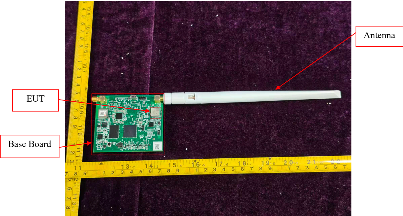
FIGURE 3 WIFI AND BLUETOOTH MODULE (M/N: LBEE5QD1ZM) BASE BOARD & EUT & ANTENNA
