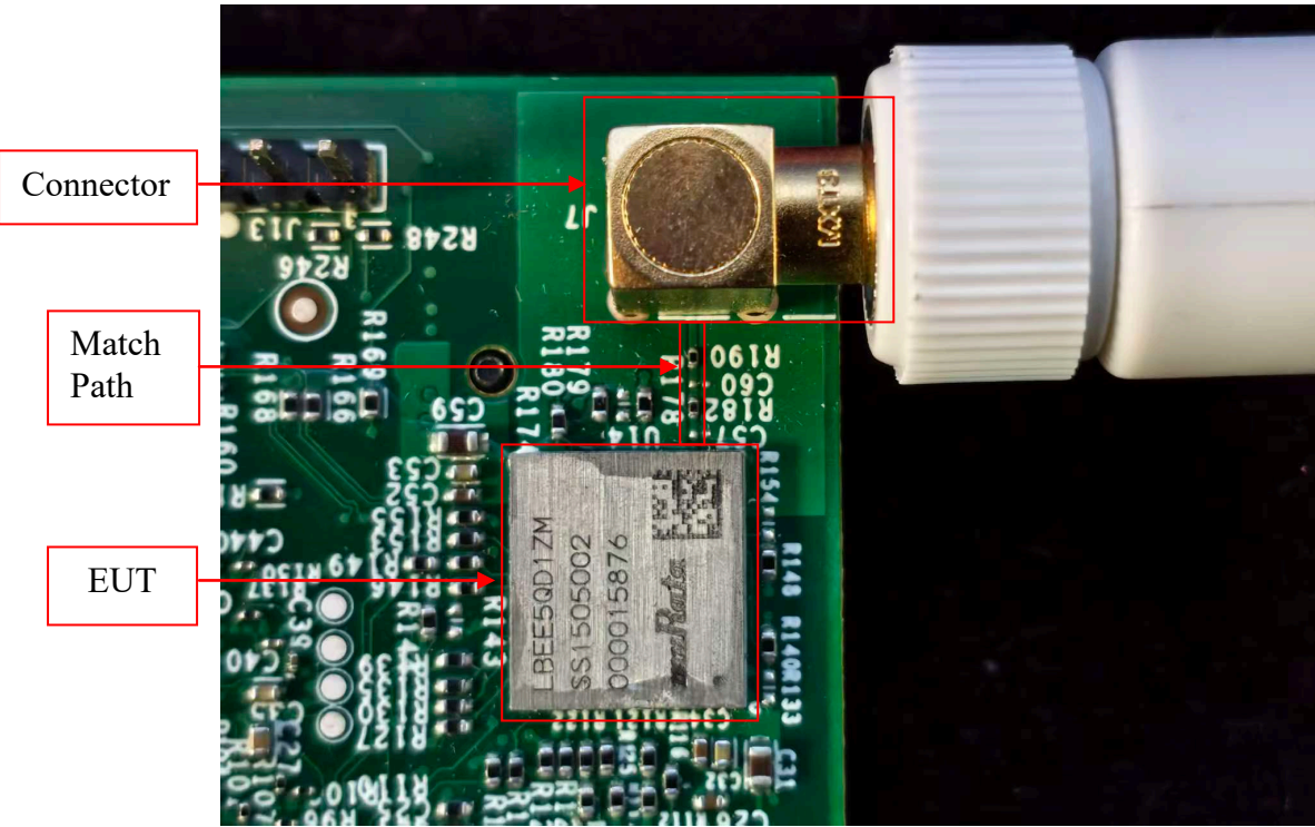
FIGURE 4 WIFI AND BLUETOOTH MODULE (M/N: LBEE5QD1ZM) EUT ON BASE BOARD
