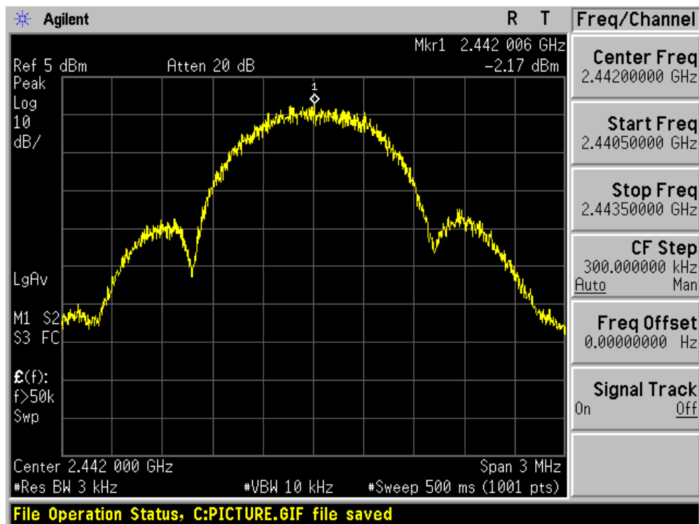
Mode 1 CH20(2442MHz)
