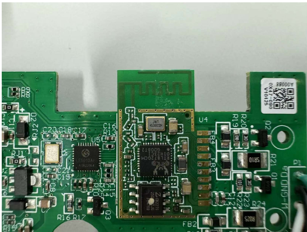
PCB view ( wireless module )
