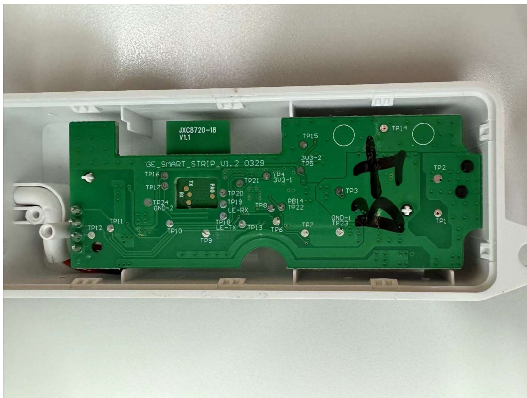
Internal view of controller
