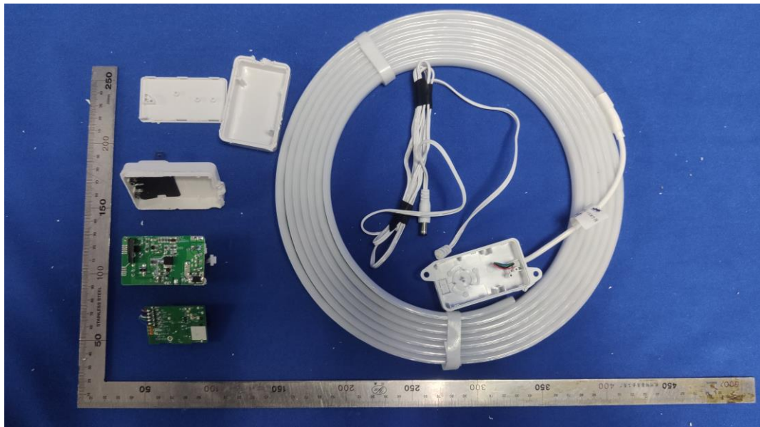
FIGURE 2 CYNCR DIRECT CONNECTED INDOOR LIGHT STRIP (16FT.) (M/N: CLEDSTR12CDIDB) COVER REMOVED #1
