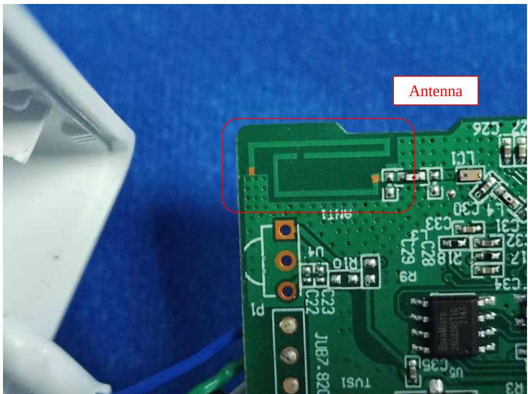
FIGURE 8 CYNC DIRECT CONNECTED INDOOR LIGHT STRIP (16FT.) (M/N: CLEDSTR12CDIDB) ANTENNA
