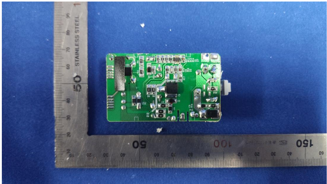
FIGURE 4 CYNCR DIRECT CONNECTED INDOOR LIGHT STRIP (16FT.) (M/N: CLEDSTR12CDIDB) POWERBOARD BACK
