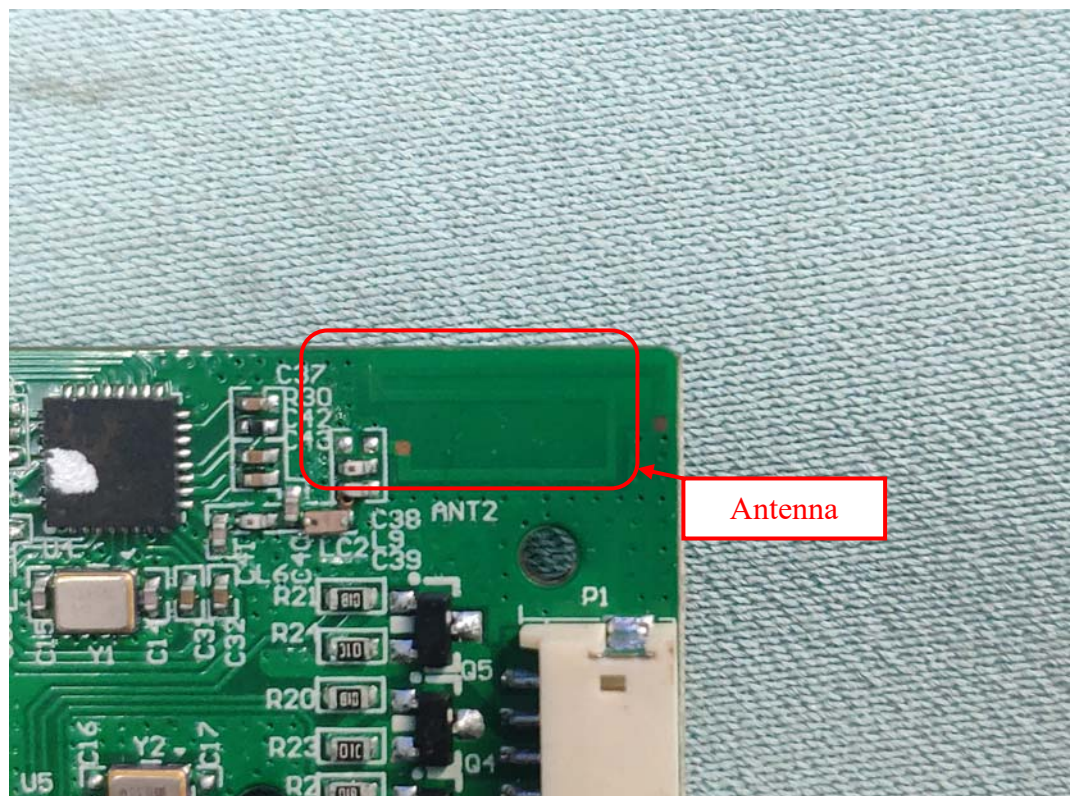
FIGURE 6 CYNCR DUAL MODE FULL COLOR LIGHT STRIP (M/N: CLEDSTR20CD1) WLAN ANT (GENERAL VIEW)
