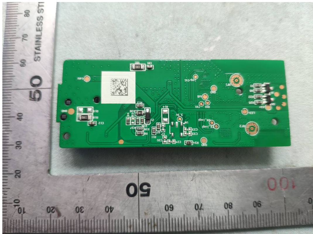
FIGURE 3 CYNIC DUAL MODE FULL COLOR LIGHT STRIP (M/N: CLEDSTR20CD1) MAIN BOARD (SOLDERED SIDE)
