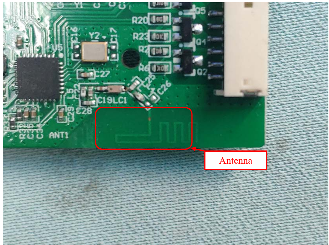
FIGURE 5 CYNCR DUAL MODE FULL COLOR LIGHT STRIP (M/N: CLEDSTR20CD1) BLE ANT (GENERAL VIEW)
