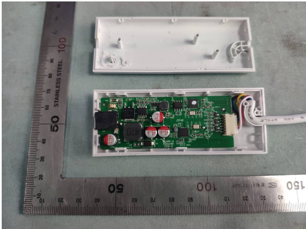
FIGURE 1 CYNCR DUAL MODE FULL COLOR LIGHT STRIP (M/N: CLEDSTR20CD1) GENERAL APPEARANCE (COVER REMOVED)
