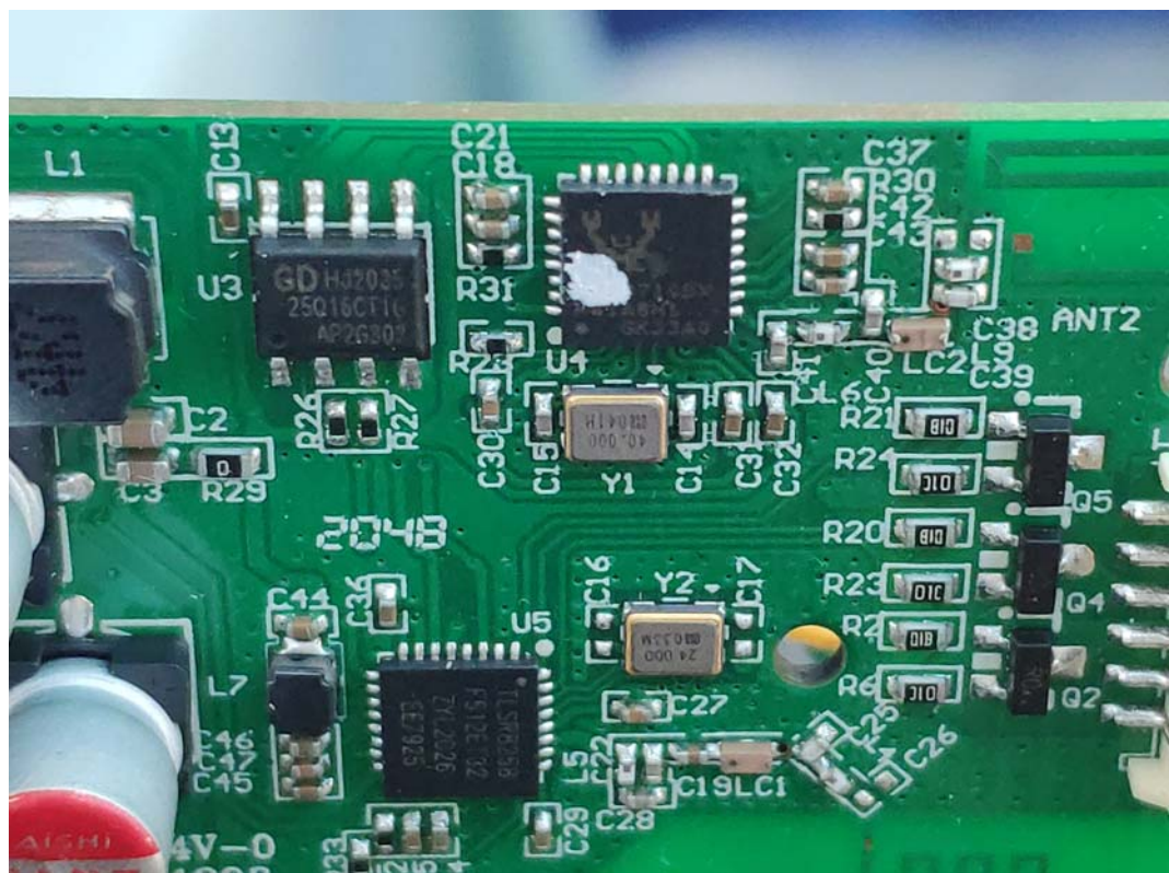
FIGURE 4 CYNIC DUAL MODE FULL COLOR LIGHT STRIP (M/N: CLEDSTR20CD1) CHIP&CRYSTAL MAIN BOARD (COMPONENT SIDE)
