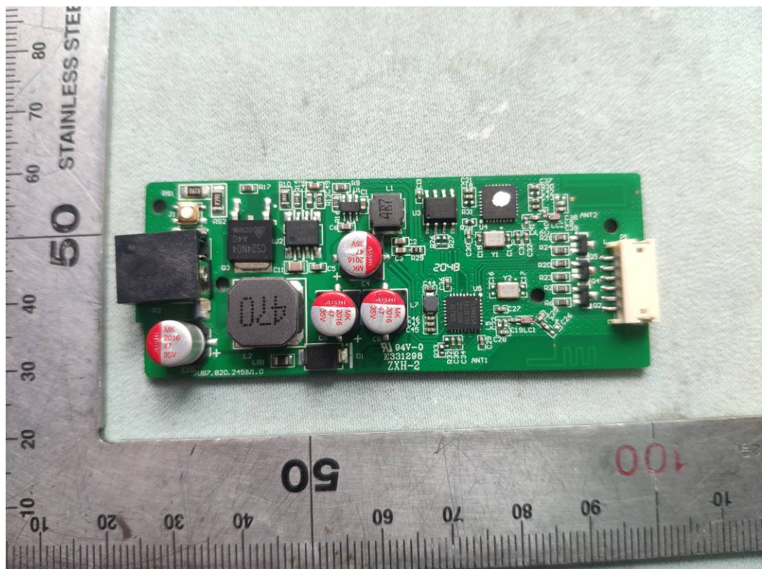
FIGURE 2 CYNCR DUAL MODE FULL COLOR LIGHT STRIP (M/N: CLEDSTR20CD1) MAIN BOARD (COMPONENT SIDE)
