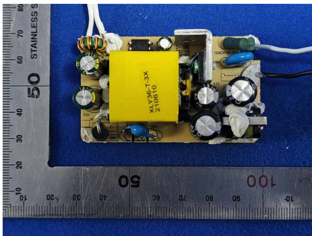
FIGURE 13 CYNCTILE (M/N: CFIHTIHCDEN) POWER BOARD FRONT
