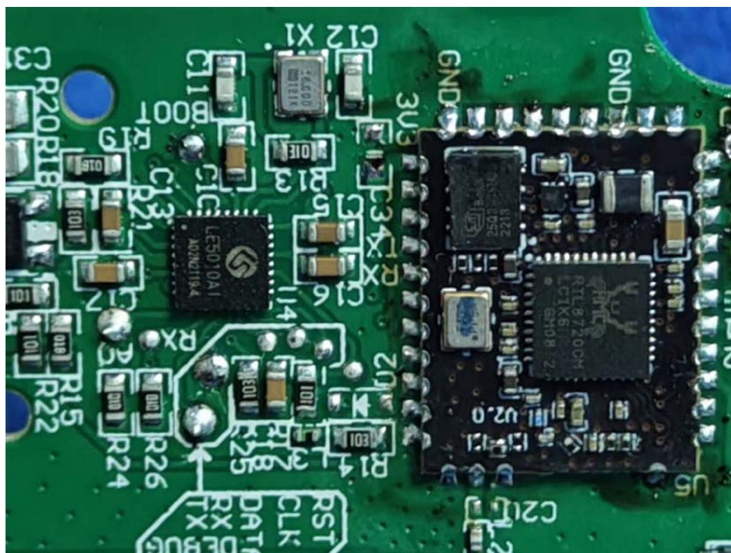
FIGURE 17 CYNCTILE (M/N: CFIXTIHCDEN) CHIP&CRYSTAL ON CONTROL BOARD
