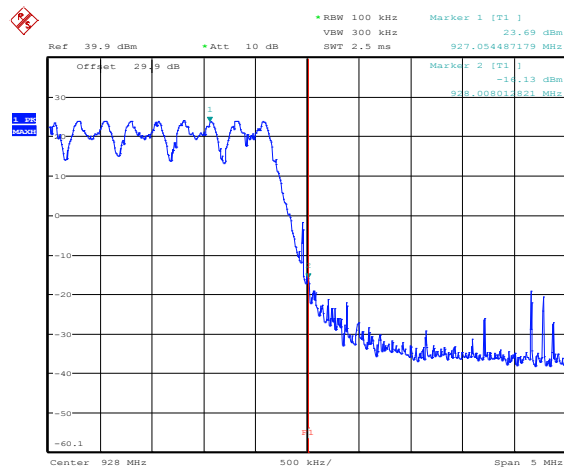
Figure 8.4-11: Upper band edge emission, tx on high channel
