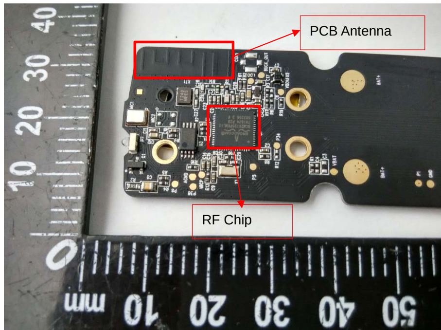
MAIN BOARD 1 TOP VIEW 2
