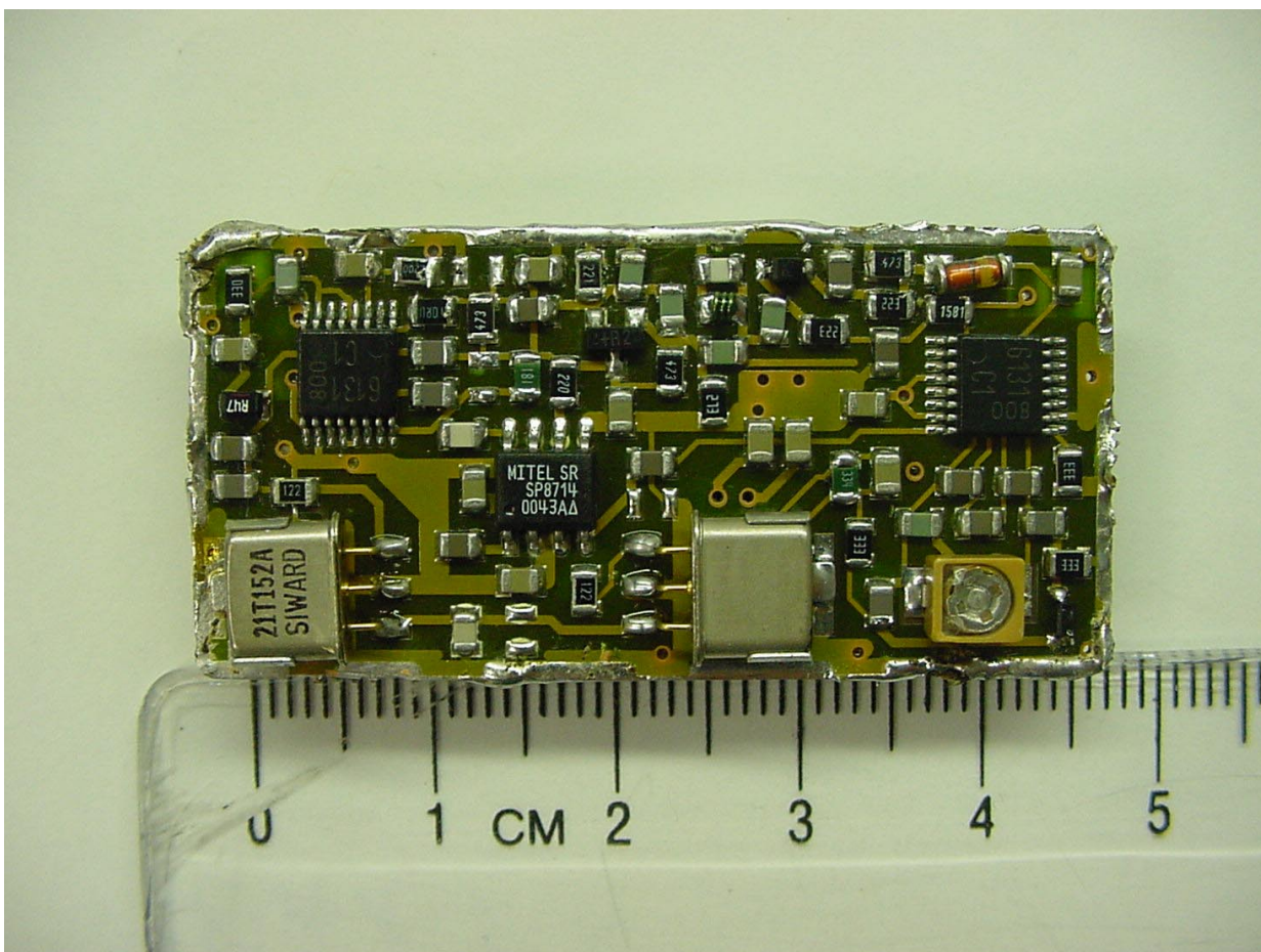
PHOTOGRAPH 14: BACK OF RECEIVER PCB
