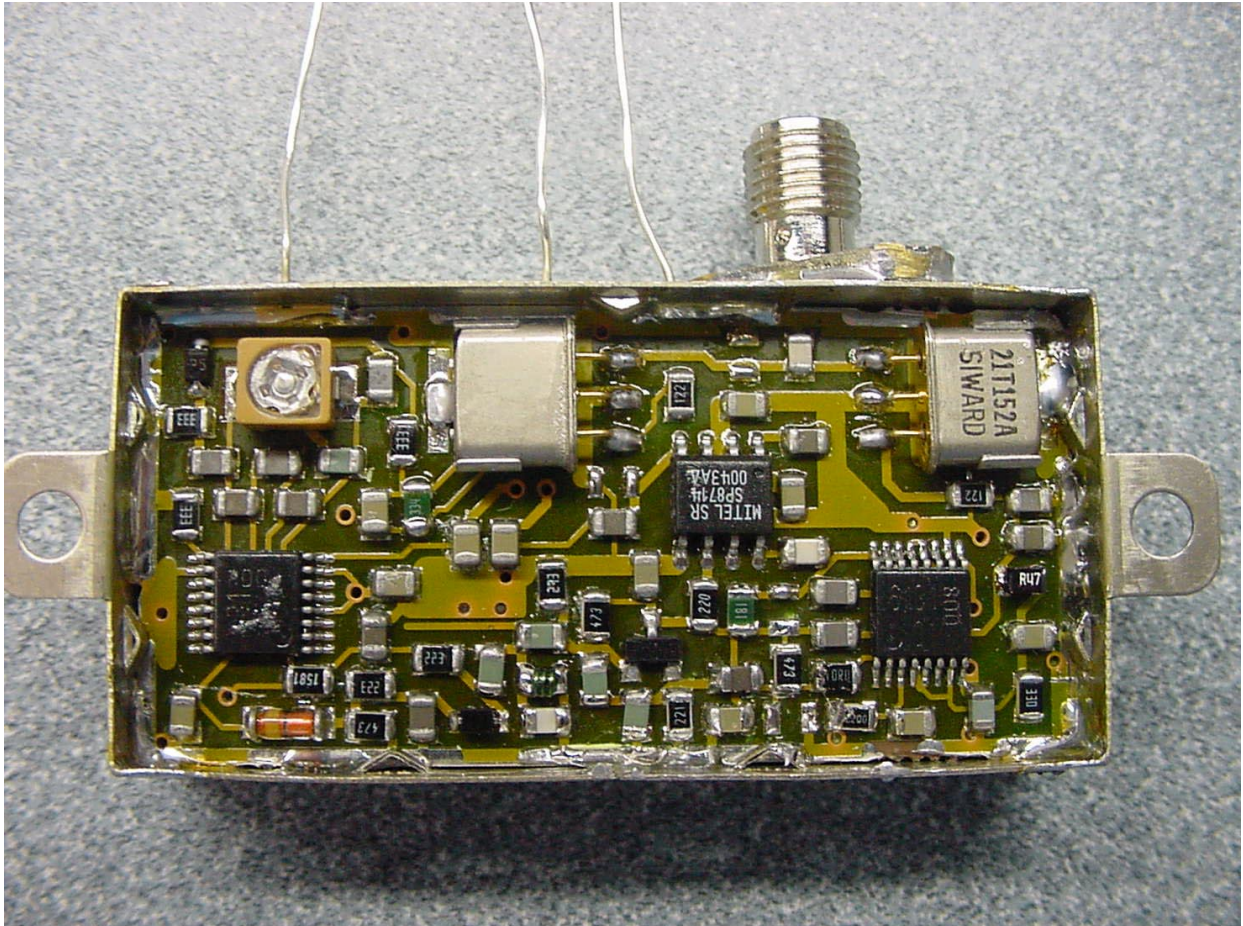
PHOTOGRAPH 13: BACK OF RECEIVER PCB IN CHASSIS
