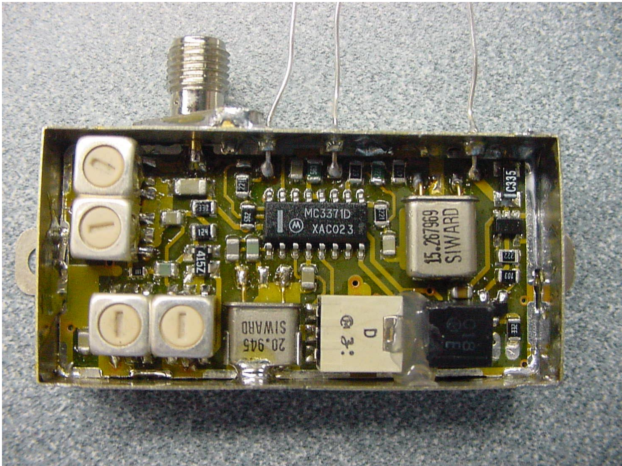
PHOTOGRAPH 15: FRONT OF RECEIVER PCB IN CHASSIS
