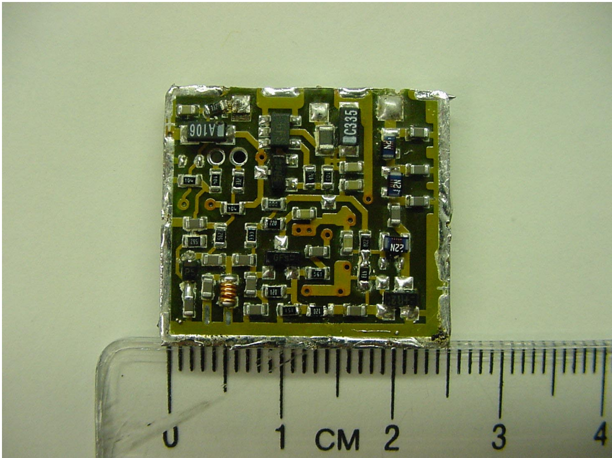
PHOTOGRAPH 24: FRONT OF TRANSMITTER PCB
