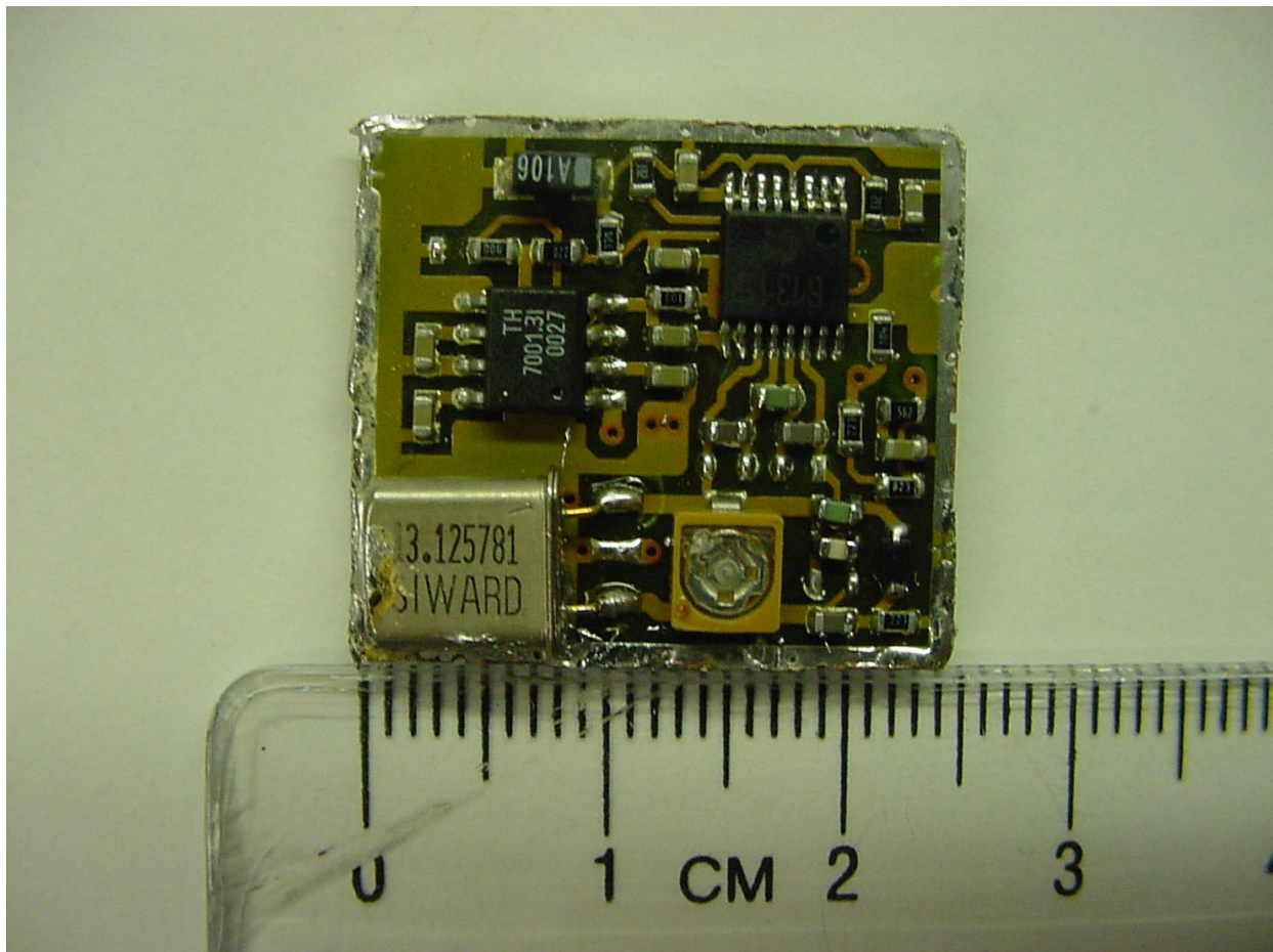
PHOTOGRAPH 26: BACK OF TRANSMITTER PCB
