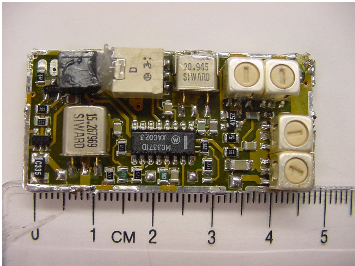
PHOTOGRAPH 30: FRONT OF RECEIVER PCB
