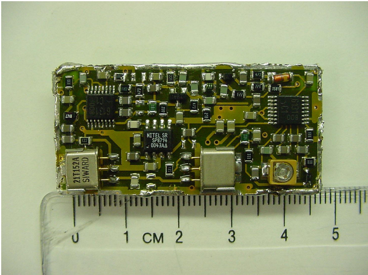
PHOTOGRAPH 28: BACK OF RECEIVER PCB
