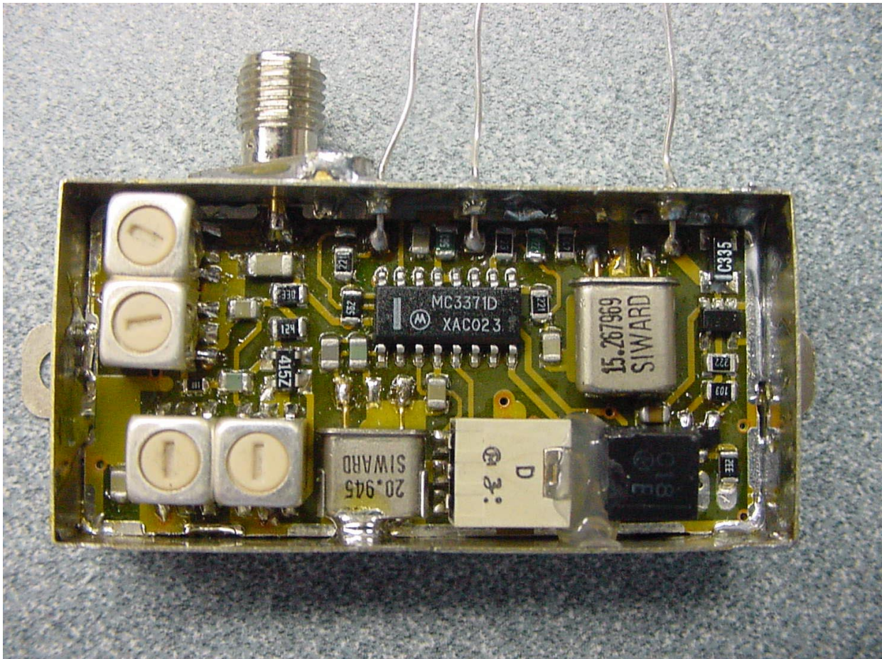
PHOTOGRAPH 29: FRONT OF RECEIVER PCB IN CHASSIS
