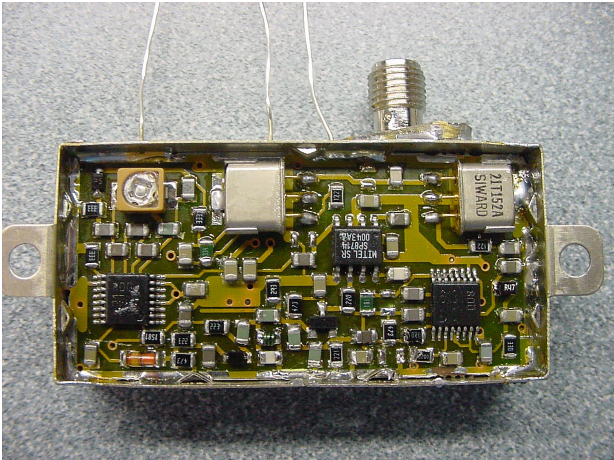
PHOTOGRAPH 27: BACK OF RECEIVER PCB IN CHASSIS
