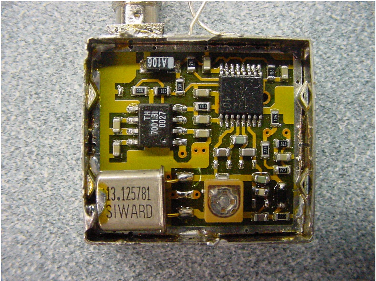
PHOTOGRAPH 25: BACK OF TRANSMITTER PCB IN CHASSIS
