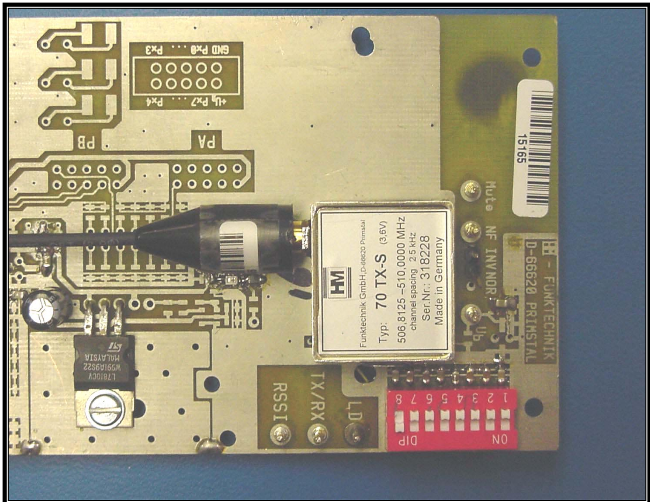
PHOTOGRAPH 11: EUT ON TEST BED PCB
