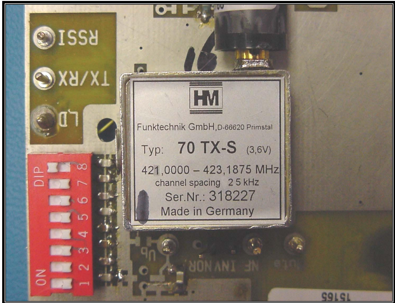
PHOTOGRAPH 4: EUT FRONT VIEW – MODULE 1
