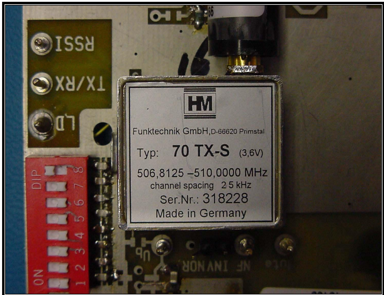
PHOTOGRAPH 6: EUT FRONT VIEW – MODULE 3
