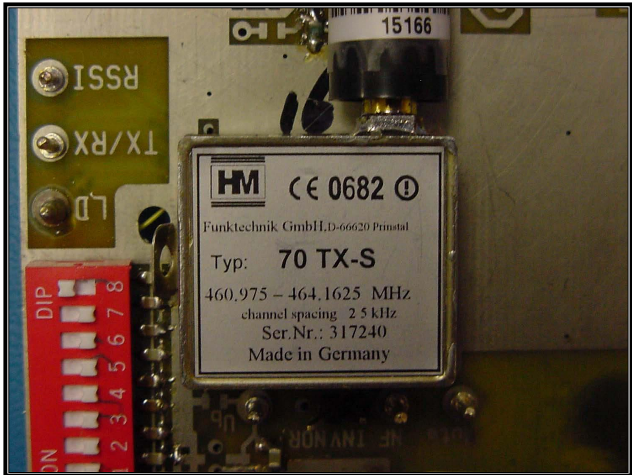
PHOTOGRAPH 5: EUT FRONT VIEW – MODULE 2
