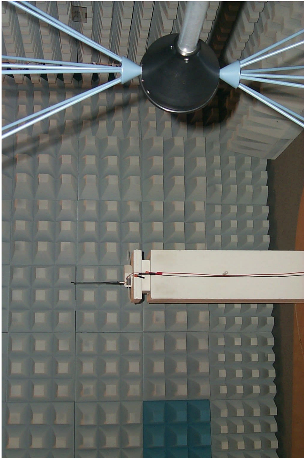
52367emi5.JPG: Test set-up radiated emissions
