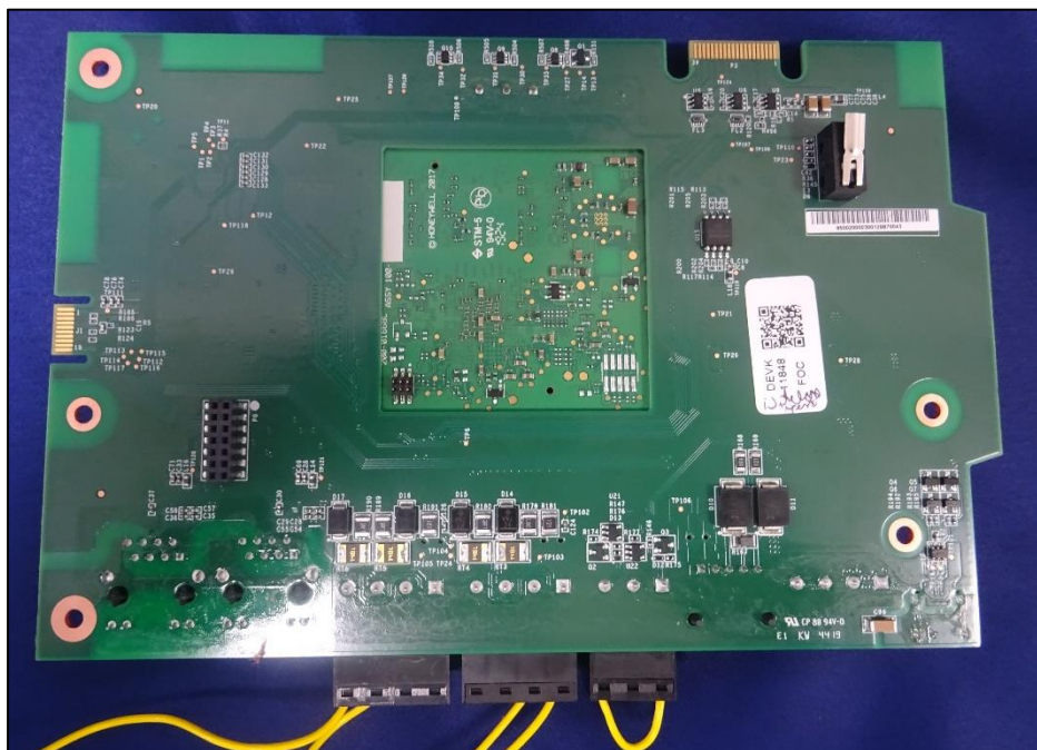
PCB Rear View
