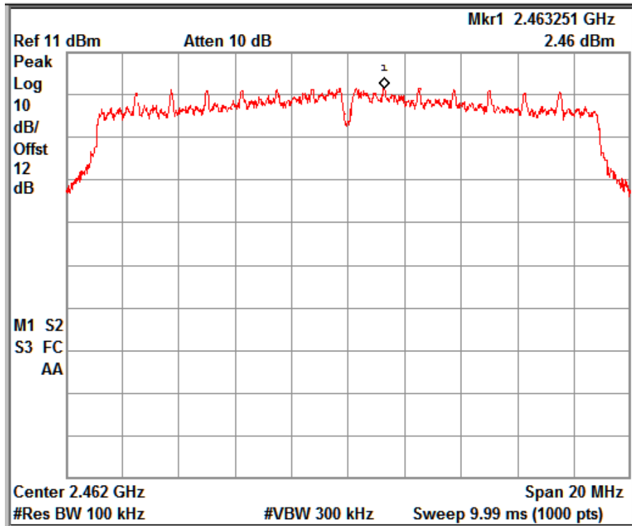
Reference Plot: MCS4, 2462MHz
