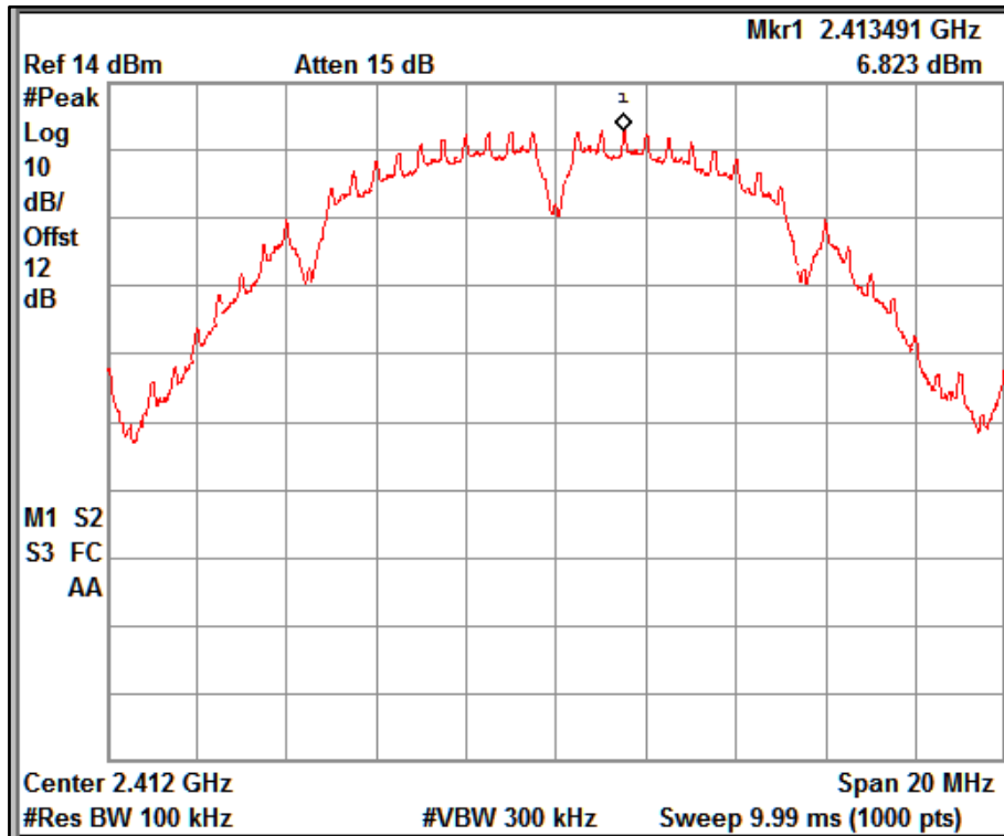
Reference Plot: 1Mbps, 2412MHz
