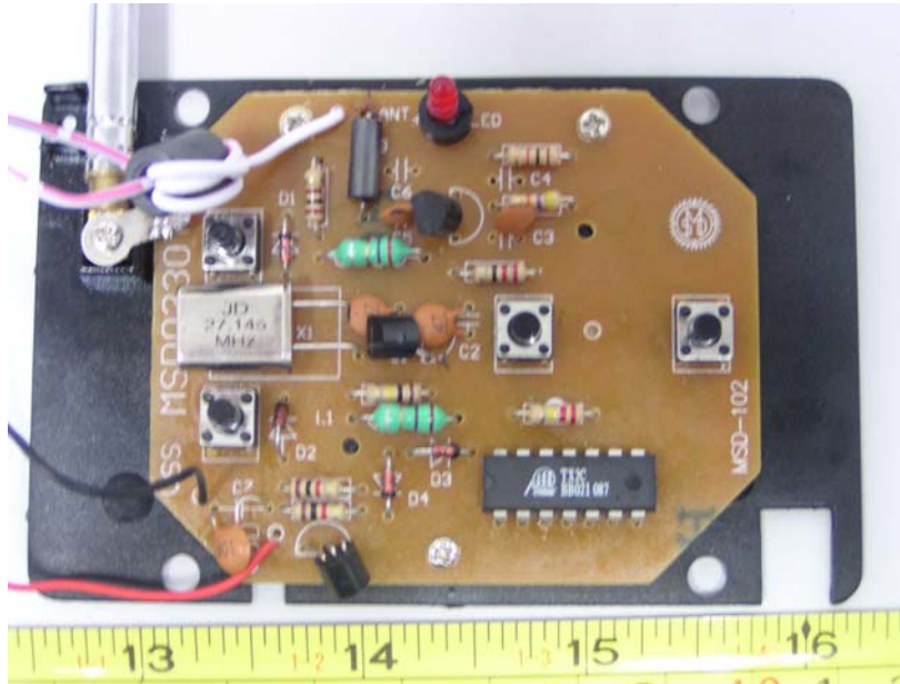
EUT – PWB – Component View
