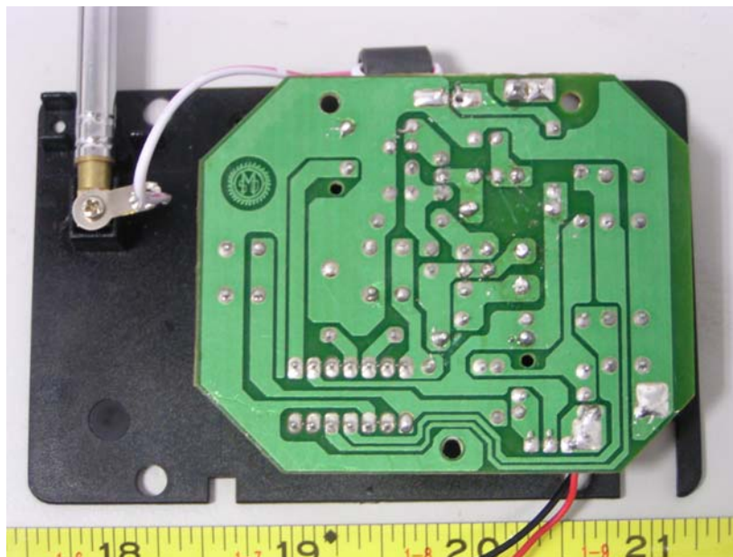
EUT –PWB – Circuit View
