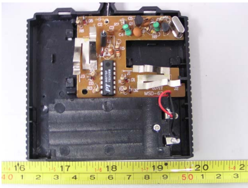
EUT – Uncovered Component view (2)
