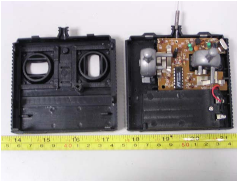
EUT – Uncovered Component view (1)
