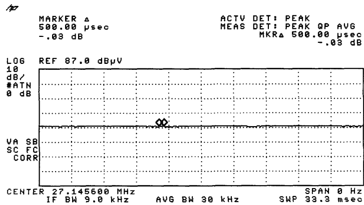
Figure C [Short Pulse]
