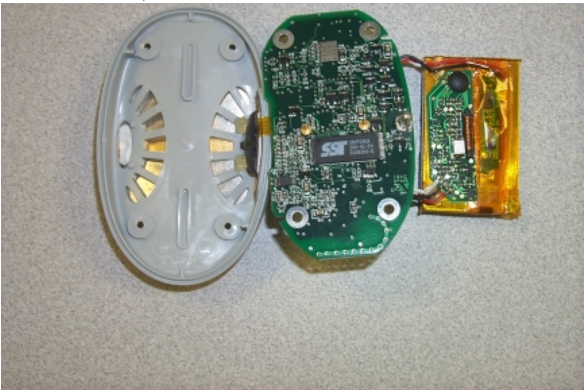
Bottom of internal chassis, Side A of internal boards
