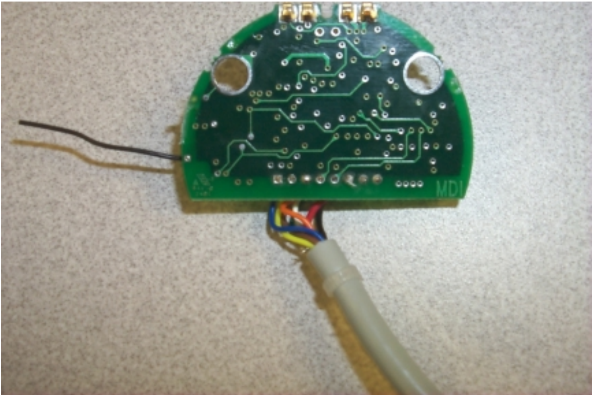
Side B of internal PC board
