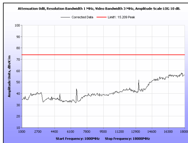
Plot 13. Radiated Spurious Emissions, Low Channel, 1 GHz – 18 GHz, Peak
