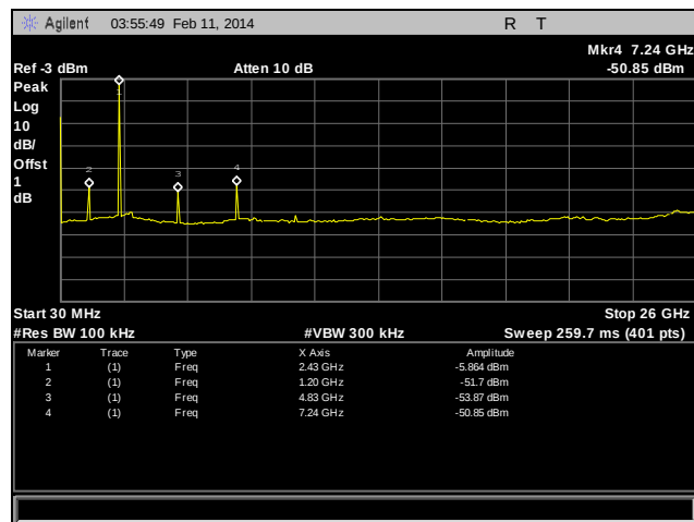
Plot 24. Conducted Spurious Emissions, Low Channel, 30 MHz – 26 GHz
