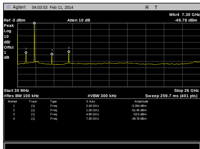
Plot 25. Conducted Spurious Emissions, Mid Channel, 30 MHz – 26 GHz
