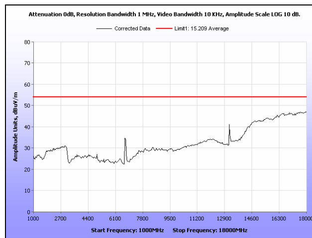
Plot 12. Radiated Spurious Emissions, Low Channel, 1 GHz – 18 GHz, Average
