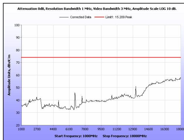
Plot 16. Radiated Spurious Emissions, Mid Channel, 1 GHz – 18 GHz, Peak
