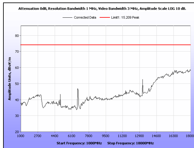
Plot 19. Radiated Spurious Emissions, High Channel, 1 GHz – 18 GHz, Peak
