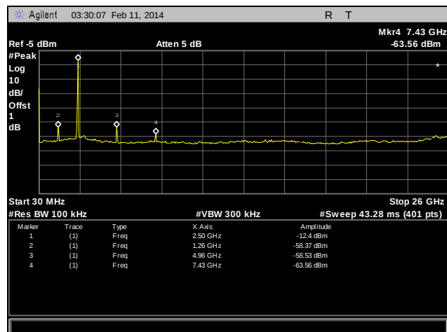
Plot 26. Conducted Spurious Emissions, High Channel, 30 MHz – 26 GHz
