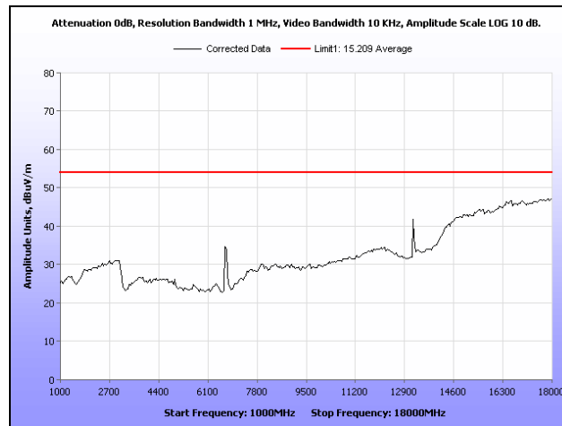
Plot 15. Radiated Spurious Emissions, Mid Channel, 1 GHz – 18 GHz, Average
