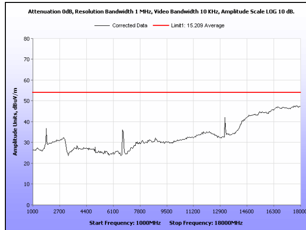
Plot 18. Radiated Spurious Emissions, High Channel, 1 GHz – 18 GHz, Average
