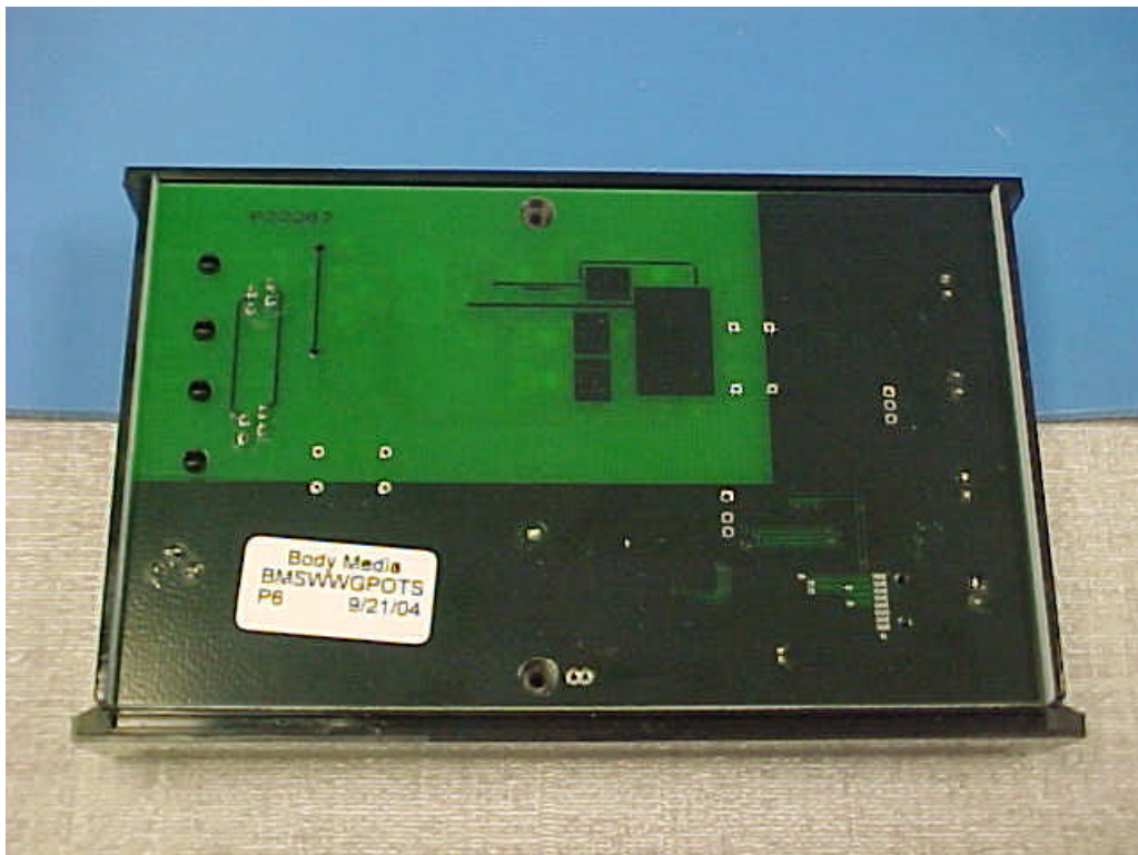
PCB bottom and enclosure
