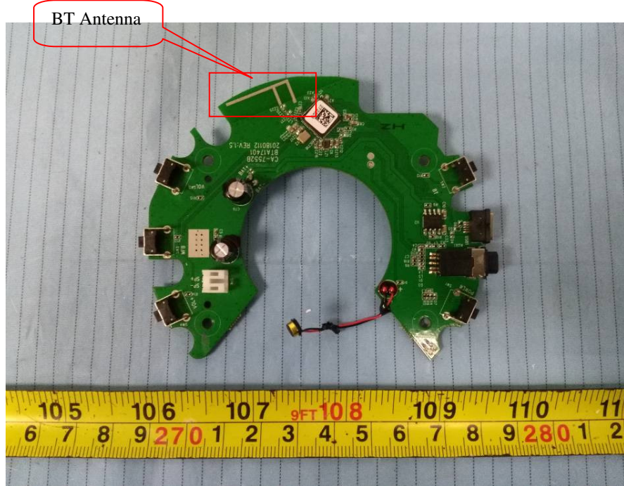
EUT –Mainboard Bottom View
