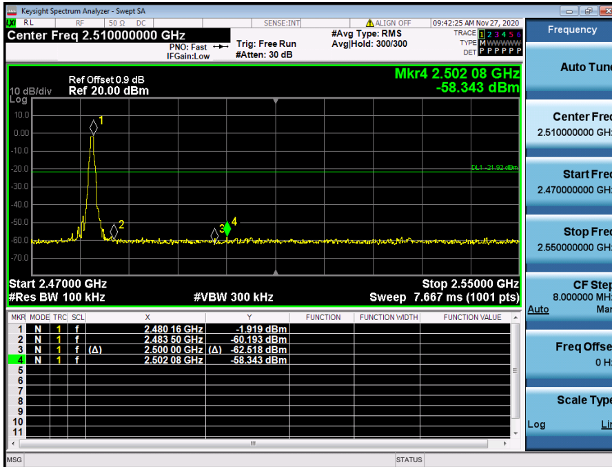
DH5_Ant1_High_2480
