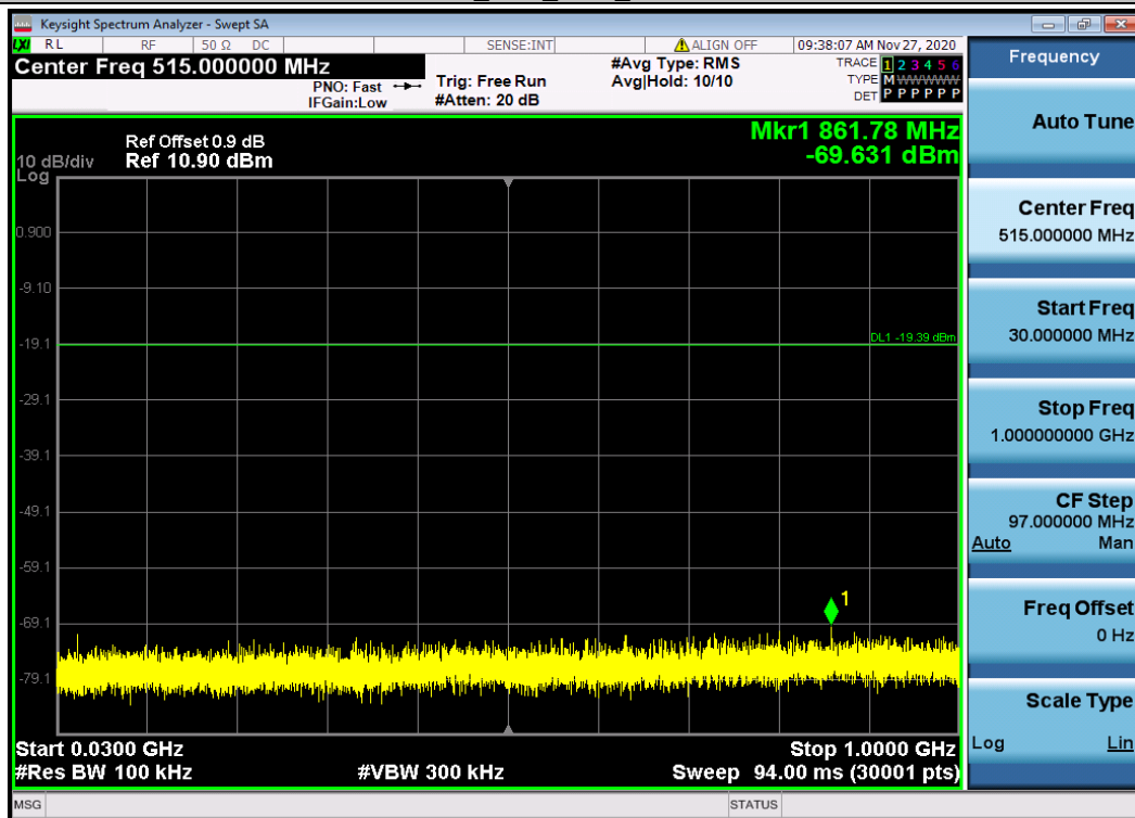
DH5_Ant1_2402_30~1000
