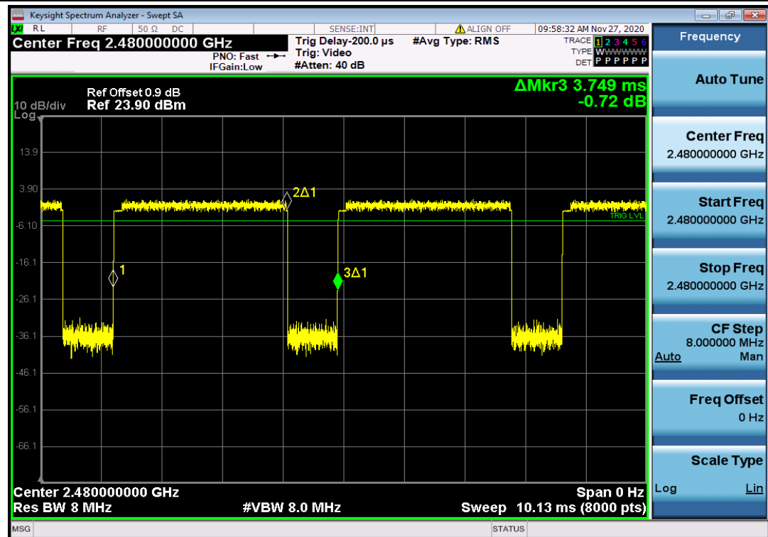
3DH5_Ant1_2480
