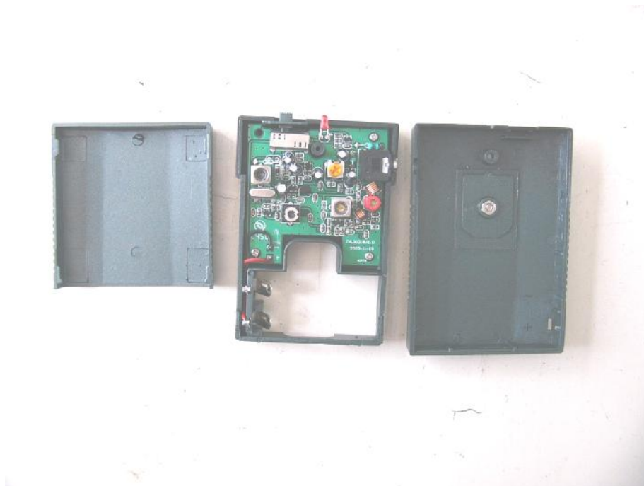
Tx EUT inside whole view
