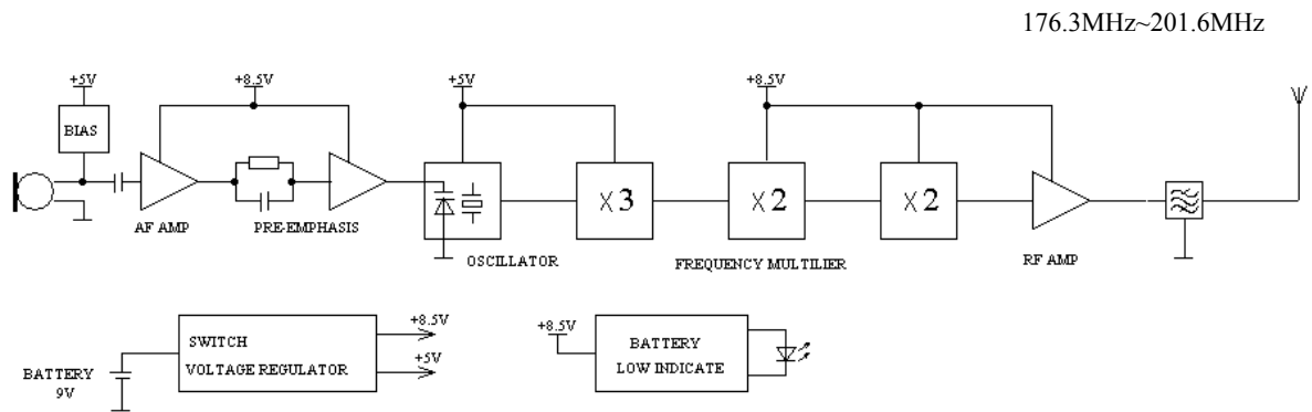
WM-737 TRANSMITTER BLOCK DIAGRAM
